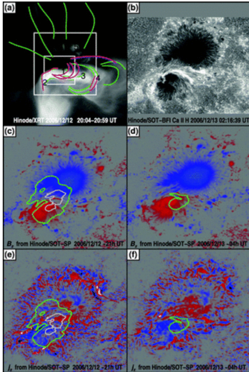
Fig. 1. from Nonlinear Forcefree Field Modeling of a Solar Active Region around the Time of a Major Flare and Coronal Mass Ejection Schrijver et al. 2008 ApJ 675 1637 doi:10.1086/527413 https://dx.doi.org/10.1086/527413 © 2008. The American Astronomical Society. All rights reserved. Printed in U.S.A.
