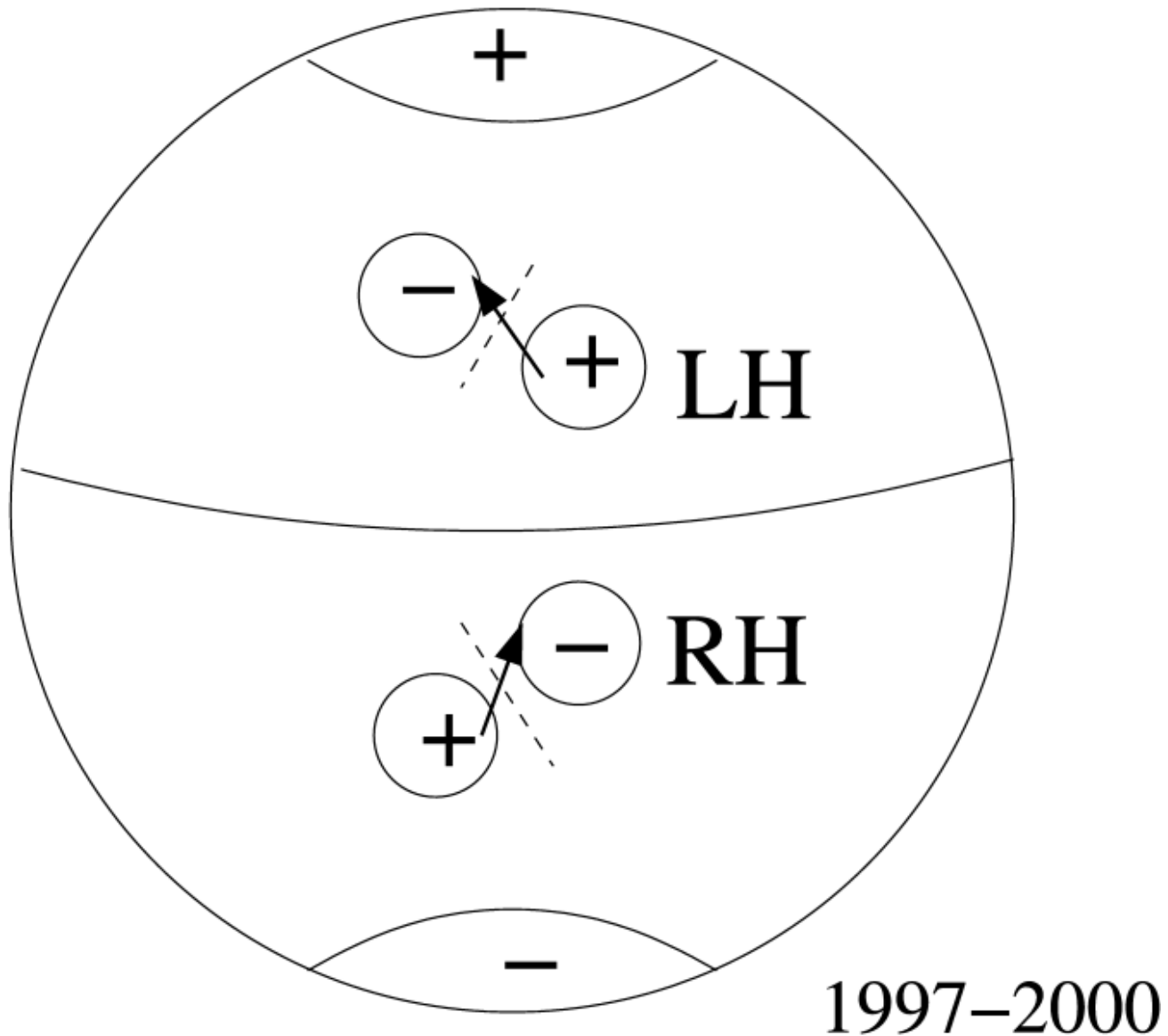
Fig. 3. from Yohkoh SXT FullResolution Observations of Sigmoids: Structure, Formation, and Eruption Canfield et al. 2007 ApJL 671 L81 doi:10.1086/524729 https://dx.doi.org/10.1086/524729 © 2007. The American Astronomical Society. All rights reserved. Printed in U.S.A.
