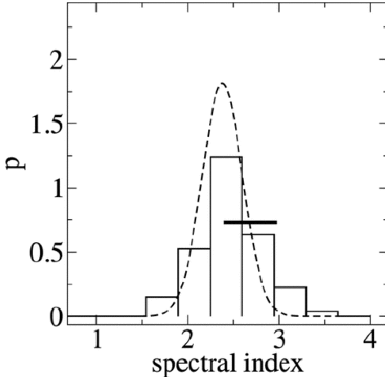
Fig. 4. from Unresolved Unidentified Source Contribution to the GammaRay Background Pavlidou et al. 2008 ApJ 677 27 doi:10.1086/524723 https://dx.doi.org/10.1086/524723 © 2008. The American Astronomical Society. All rights reserved. Printed in U.S.A.
