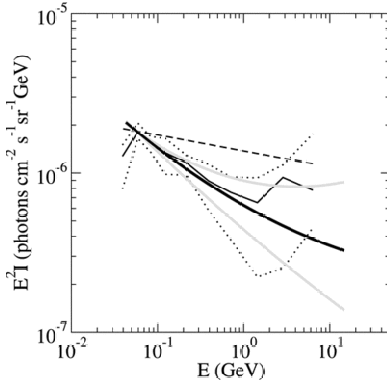
Fig. 3. from Unresolved Unidentified Source Contribution to the GammaRay Background Pavlidou et al. 2008 ApJ 677 27 doi:10.1086/524723 https://dx.doi.org/10.1086/524723 © 2008. The American Astronomical Society. All rights reserved. Printed in U.S.A.
