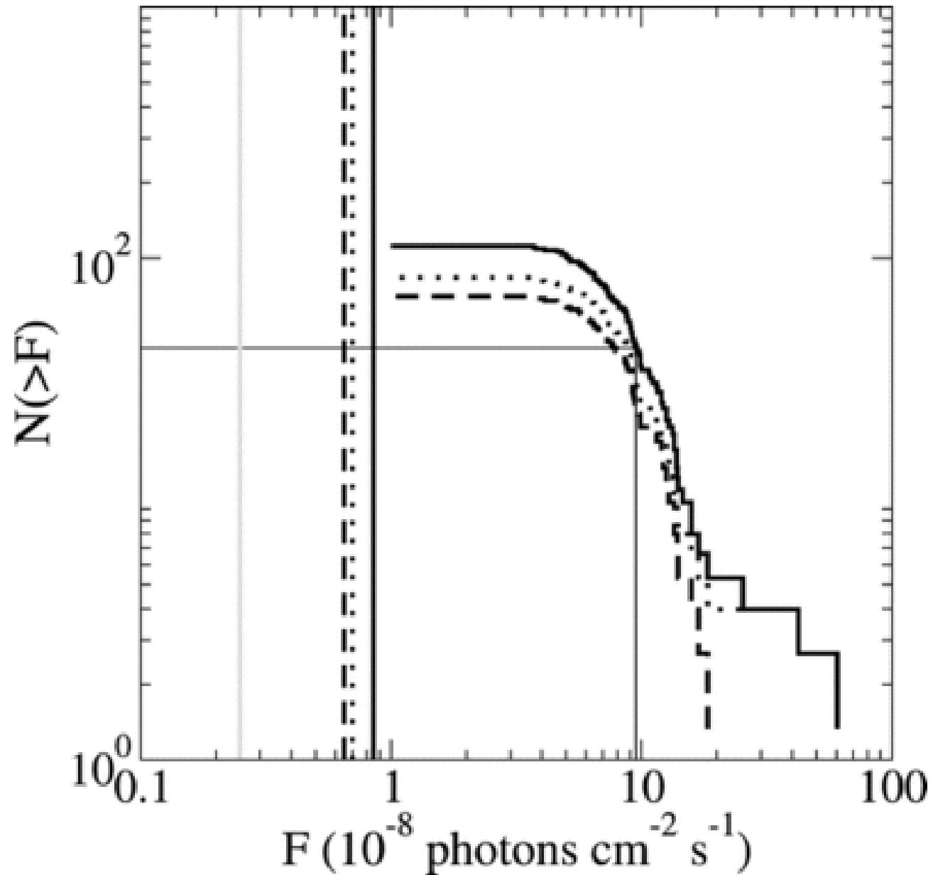
Fig. 2. from Unresolved Unidentified Source Contribution to the GammaRay Background Pavlidou et al. 2008 ApJ 677 27 doi:10.1086/524723 https://dx.doi.org/10.1086/524723 © 2008. The American Astronomical Society. All rights reserved. Printed in U.S.A.
