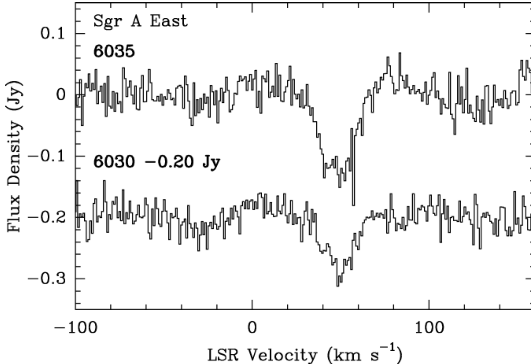
Fig. 2. from Effelsberg Observations of ExcitedState (6.0 GHz) OH in Supernova Remnants and W3(OH) Fish, Sjouwerman, & Pihlström 2007 ApJL 670 L117 doi:10.1086/524196 https://dx.doi.org/10.1086/524196 © 2007. The American Astronomical Society. All rights reserved. Printed in U.S.A.
