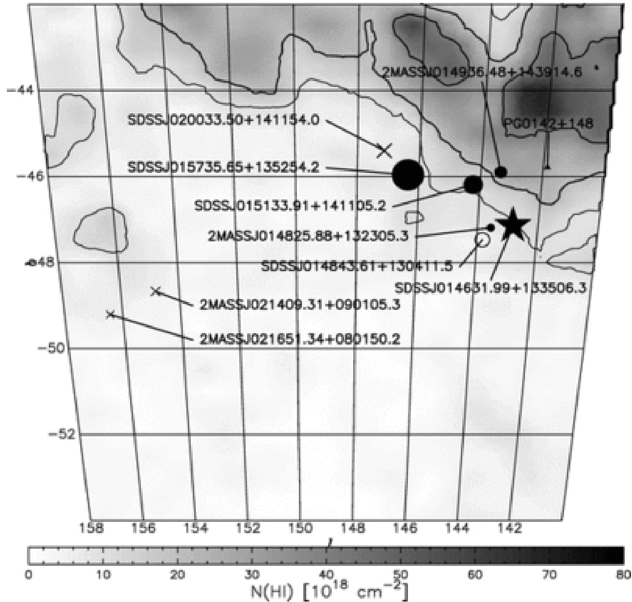
Fig. 4. from Distances to Galactic HighVelocity Clouds. I. Cohen Stream, Complex GCP, Cloud g1 Wakker et al. 2008 ApJ 672 298 doi:10.1086/523845 https://dx.doi.org/10.1086/523845 © 2008. The American Astronomical Society. All rights reserved. Printed in U.S.A.
