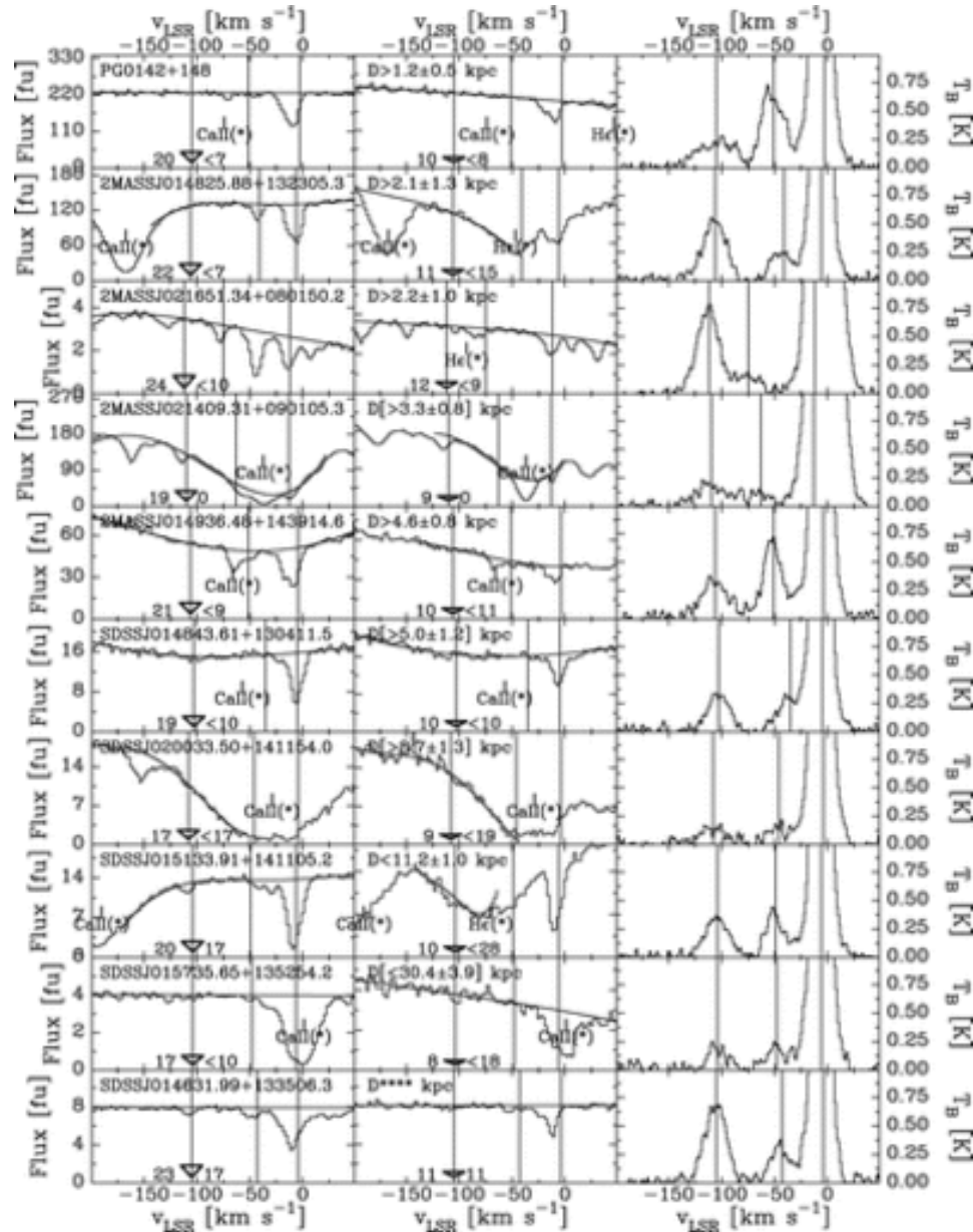
Fig. 3. from Distances to Galactic HighVelocity Clouds. I. Cohen Stream, Complex GCP, Cloud g1 Wakker et al. 2008 ApJ 672 298 doi:10.1086/523845 https://dx.doi.org/10.1086/523845
