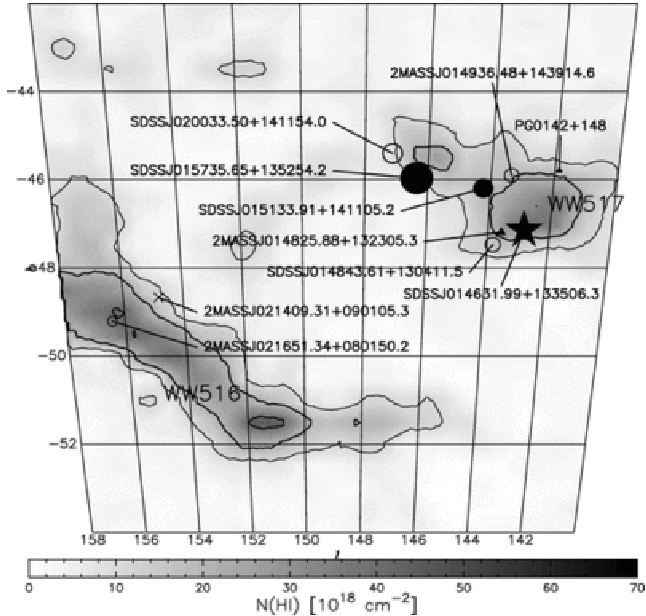
Fig. 2. from Distances to Galactic HighVelocity Clouds. I. Cohen Stream, Complex GCP, Cloud g1 Wakker et al. 2008 ApJ 672 298 doi:10.1086/523845 https://dx.doi.org/10.1086/523845 © 2008. The American Astronomical Society. All rights reserved. Printed in U.S.A.
