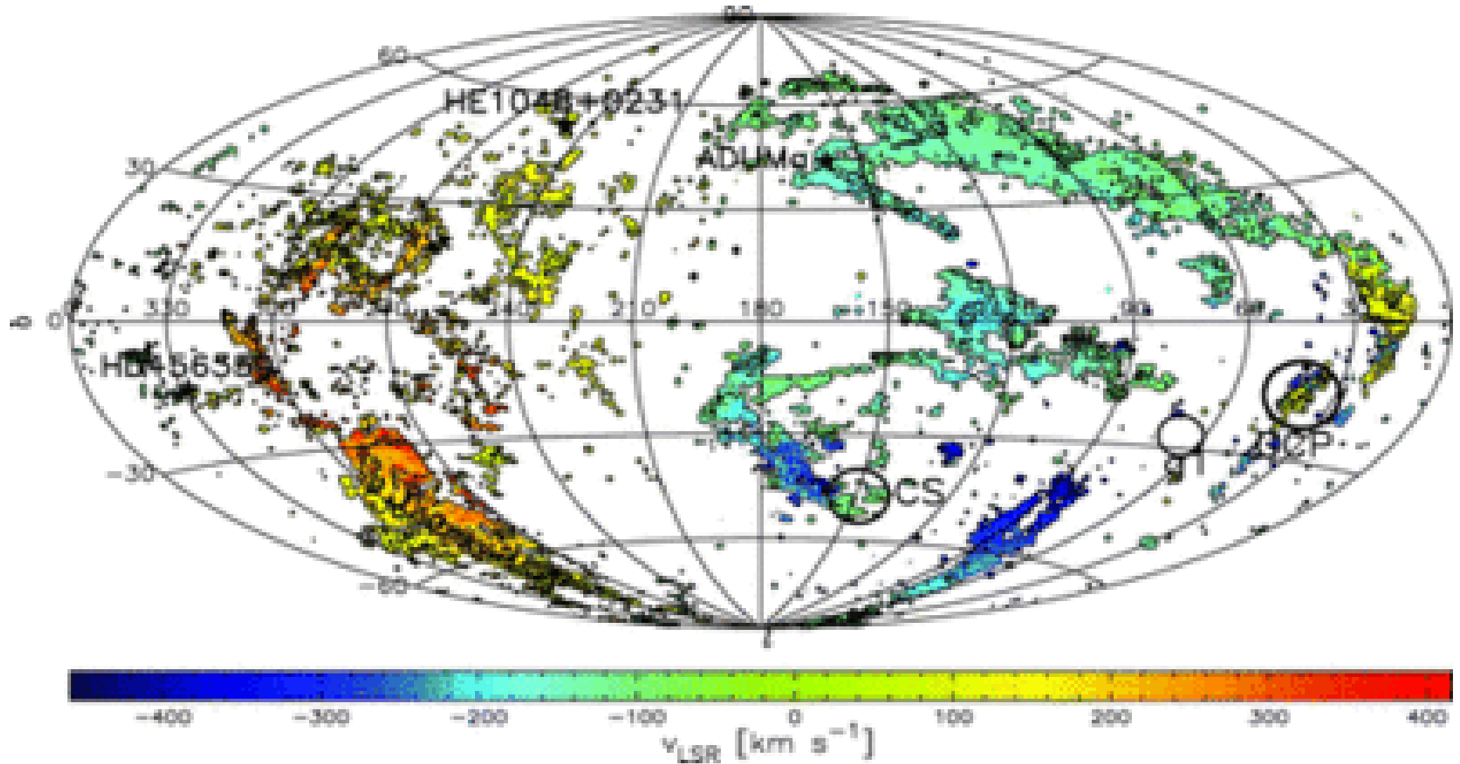
Fig. 1. from Distances to Galactic HighVelocity Clouds. I. Cohen Stream, Complex GCP, Cloud g1 Wakker et al. 2008 ApJ 672 298 doi:10.1086/523845 https://dx.doi.org/10.1086/523845 © 2008. The American Astronomical Society. All rights reserved. Printed in U.S.A.
