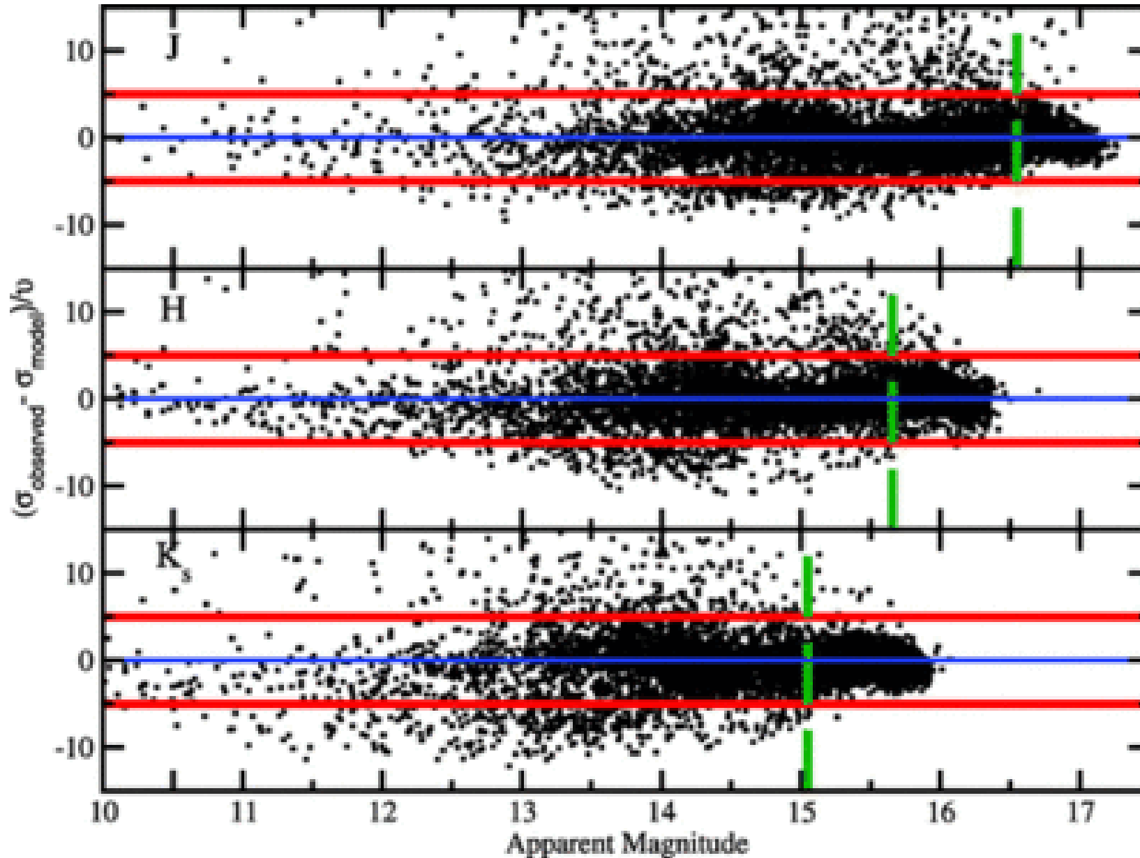
Fig. 9. from NearInfrared Variability in the 2MASS Calibration Fields: A Search for Planetary Transit Candidates Plavchan et al. 2008 ApJS 175 191 doi:10.1086/523644 https://dx.doi.org/10.1086/523644 © 2008. The American Astronomical Society. All rights reserved. Printed in U.S.A.
