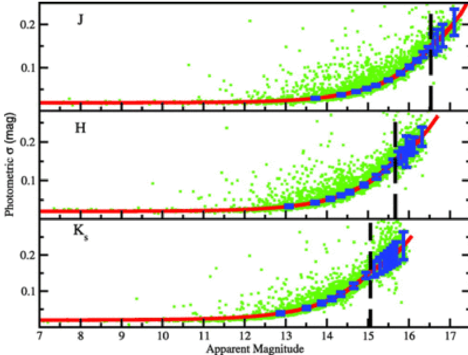
Fig. 8. from NearInfrared Variability in the 2MASS Calibration Fields: A Search for Planetary Transit Candidates Plavchan et al. 2008 ApJS 175 191 doi:10.1086/523644 https://dx.doi.org/10.1086/523644 © 2008. The American Astronomical Society. All rights reserved. Printed in U.S.A.
