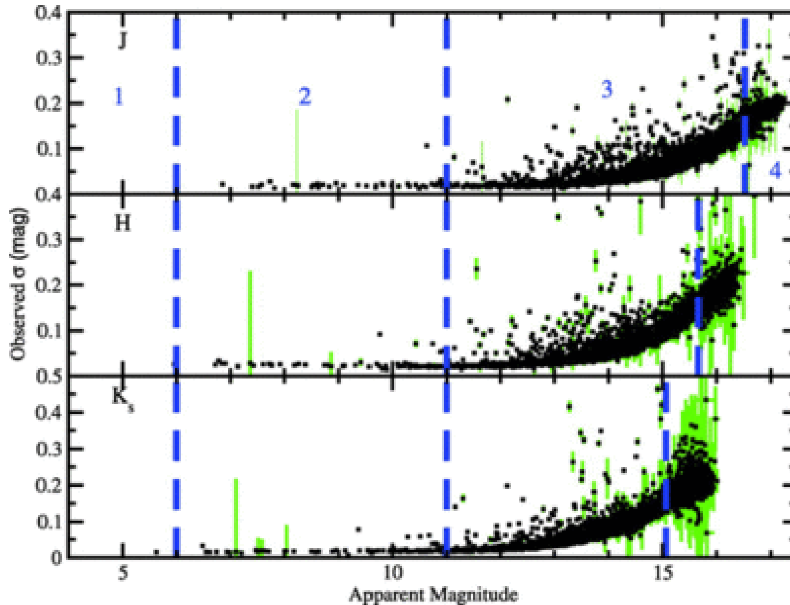
Fig. 7. from NearInfrared Variability in the 2MASS Calibration Fields: A Search for Planetary Transit Candidates Plavchan et al. 2008 ApJS 175 191 doi:10.1086/523644 https://dx.doi.org/10.1086/523644
