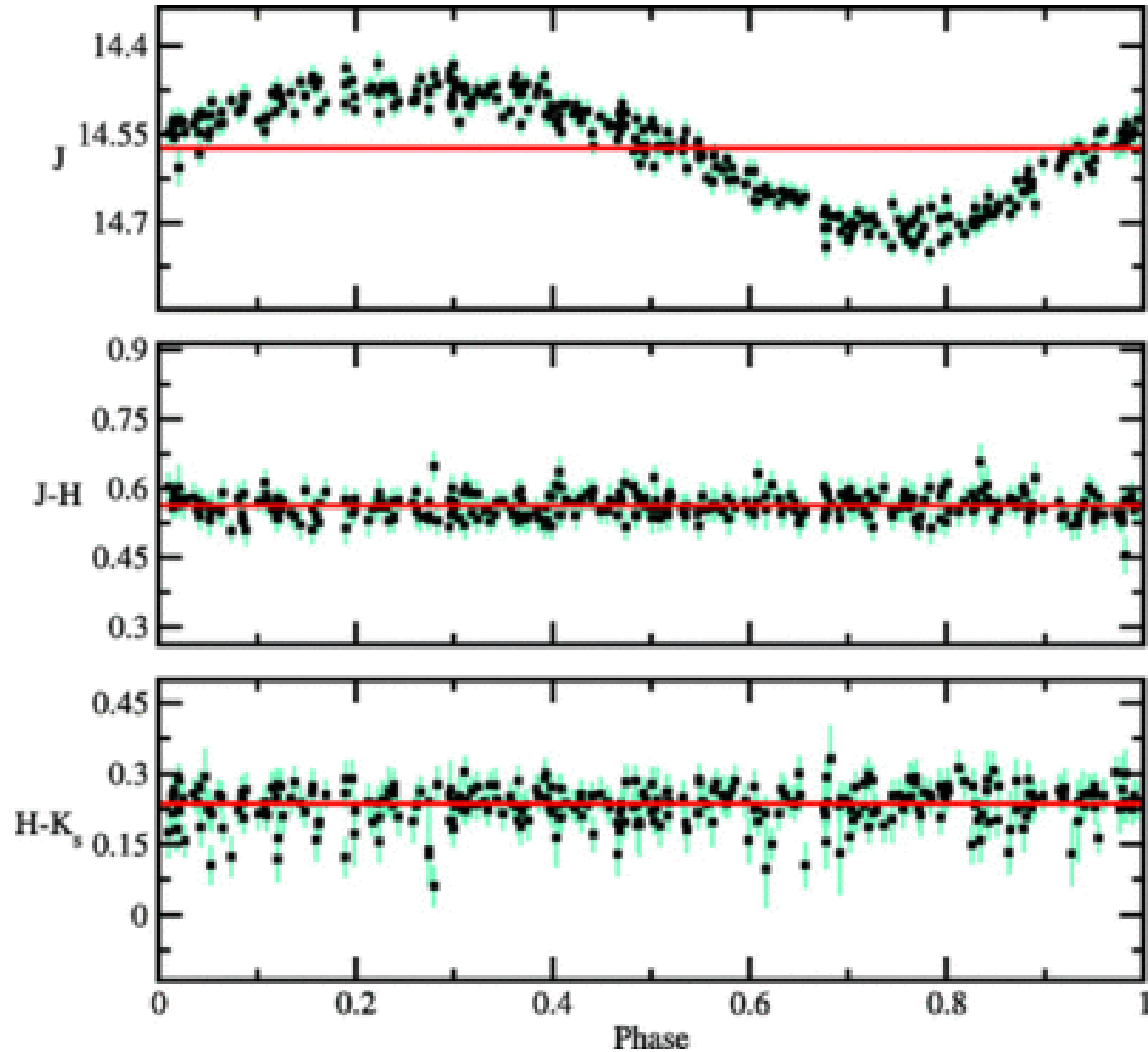
Fig. 65. from NearInfrared Variability in the 2MASS Calibration Fields: A Search for Planetary Transit Candidates Plavchan et al. 2008 ApJS 175 191 doi:10.1086/523644 https://dx.doi.org/10.1086/523644
