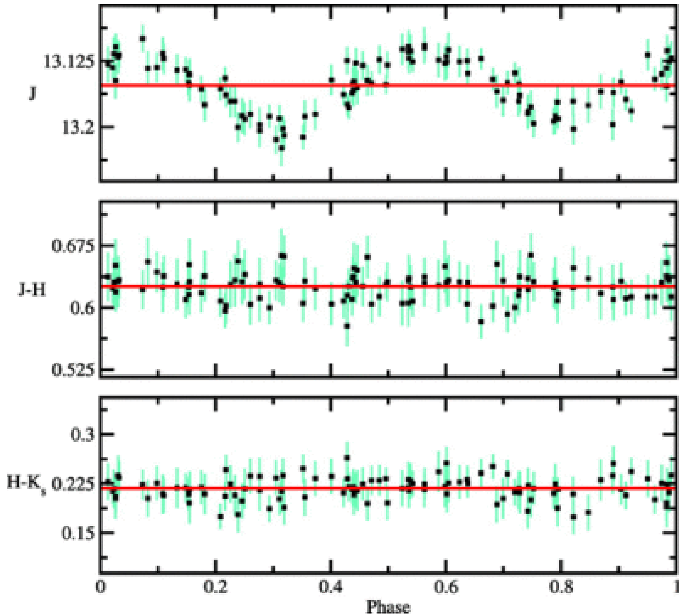
Fig. 62. from NearInfrared Variability in the 2MASS Calibration Fields: A Search for Planetary Transit Candidates Plavchan et al. 2008 ApJS 175 191 doi:10.1086/523644 https://dx.doi.org/10.1086/523644 © 2008. The American Astronomical Society. All rights reserved. Printed in U.S.A.
