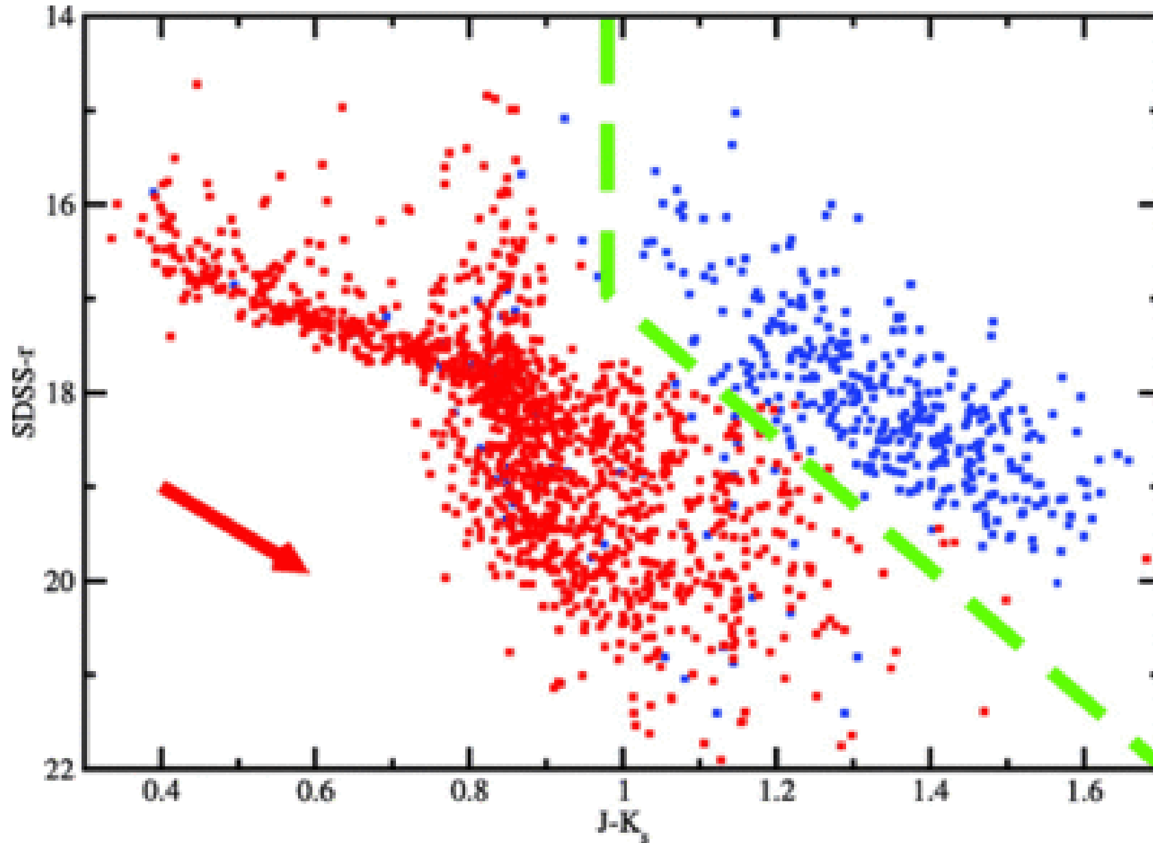
Fig. 6. from NearInfrared Variability in the 2MASS Calibration Fields: A Search for Planetary Transit Candidates Plavchan et al. 2008 ApJS 175 191 doi:10.1086/523644 https://dx.doi.org/10.1086/523644
