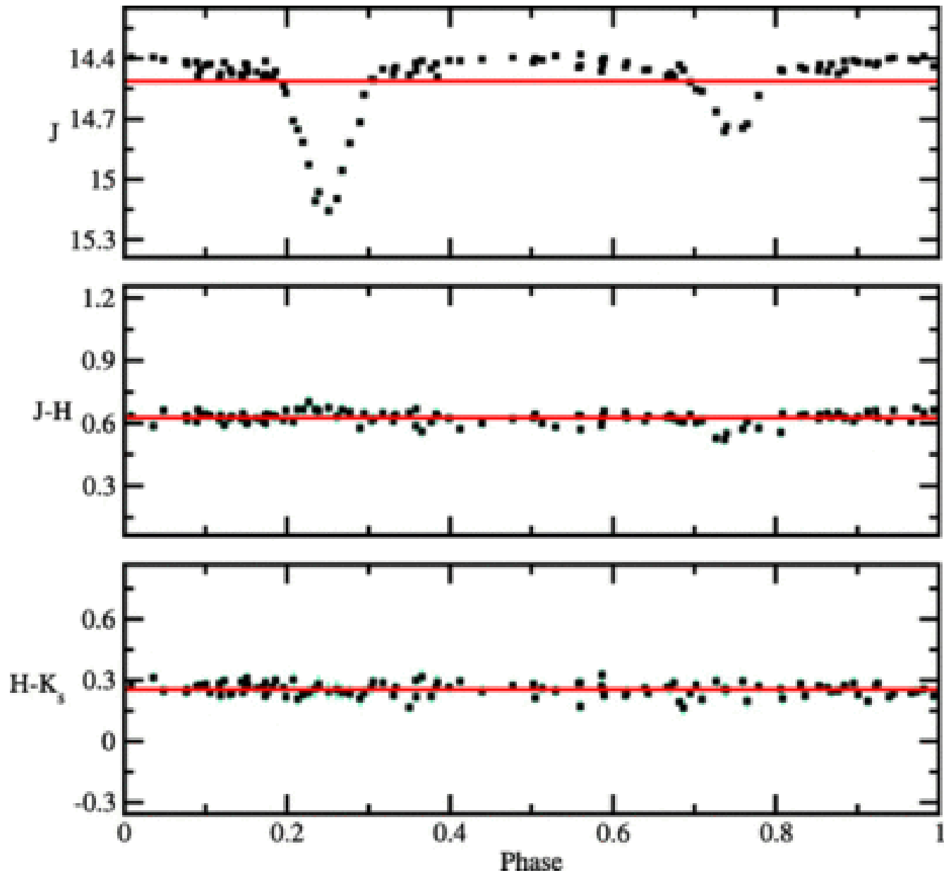
Fig. 59. from NearInfrared Variability in the 2MASS Calibration Fields: A Search for Planetary Transit Candidates Plavchan et al. 2008 ApJS 175 191 doi:10.1086/523644 https://dx.doi.org/10.1086/523644
