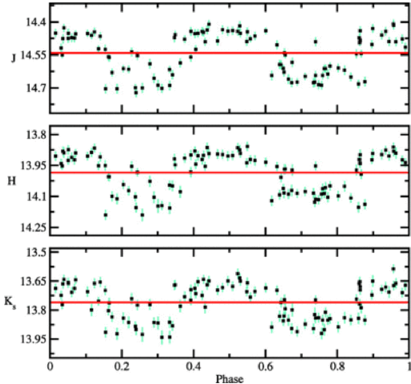
Fig. 34. from NearInfrared Variability in the 2MASS Calibration Fields: A Search for Planetary Transit Candidates Plavchan et al. 2008 ApJS 175 191 doi:10.1086/523644 https://dx.doi.org/10.1086/523644 © 2008. The American Astronomical Society. All rights reserved. Printed in U.S.A.
