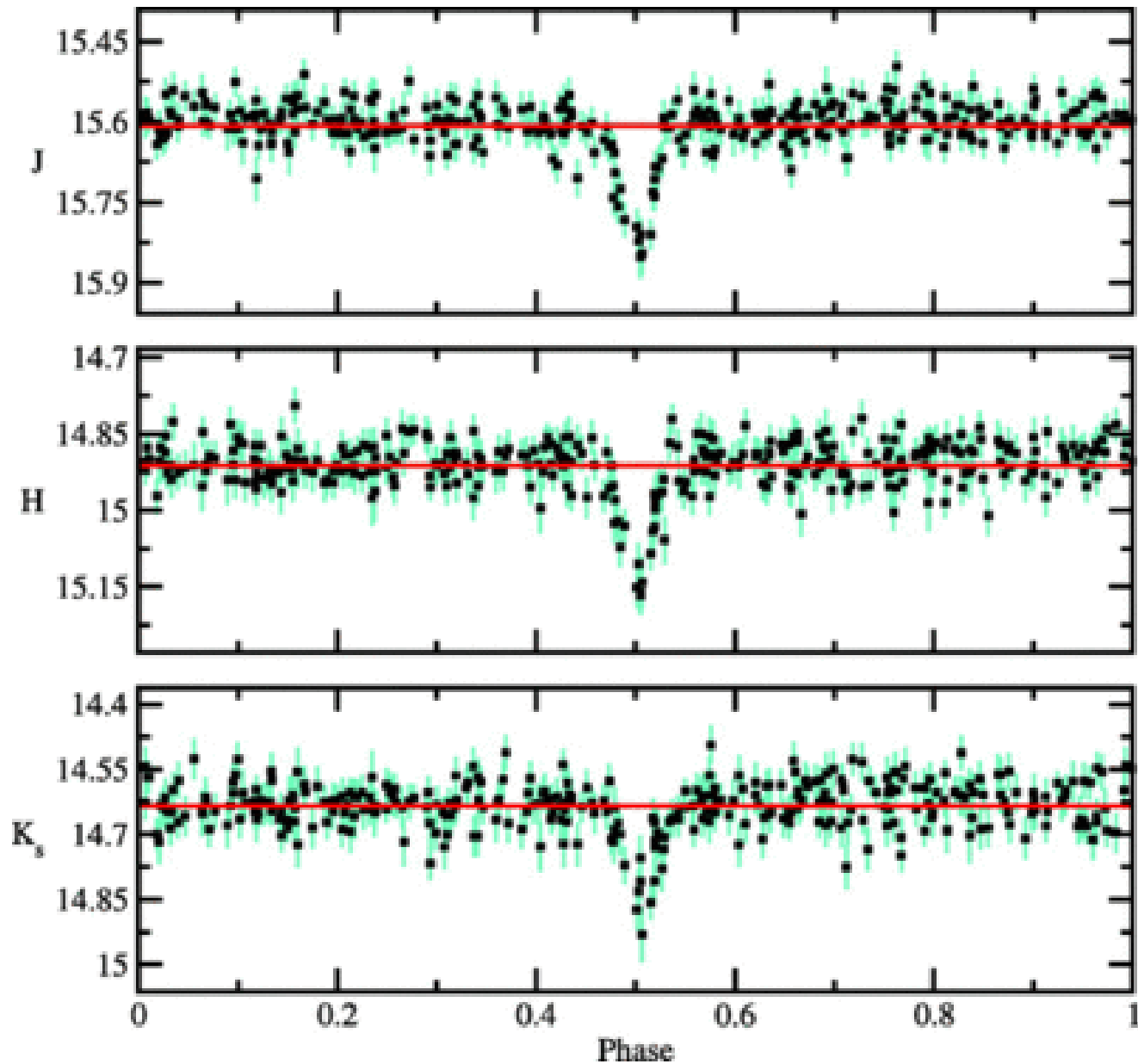
Fig. 24. from NearInfrared Variability in the 2MASS Calibration Fields: A Search for Planetary Transit Candidates Plavchan et al. 2008 ApJS 175 191 doi:10.1086/523644 https://dx.doi.org/10.1086/523644
