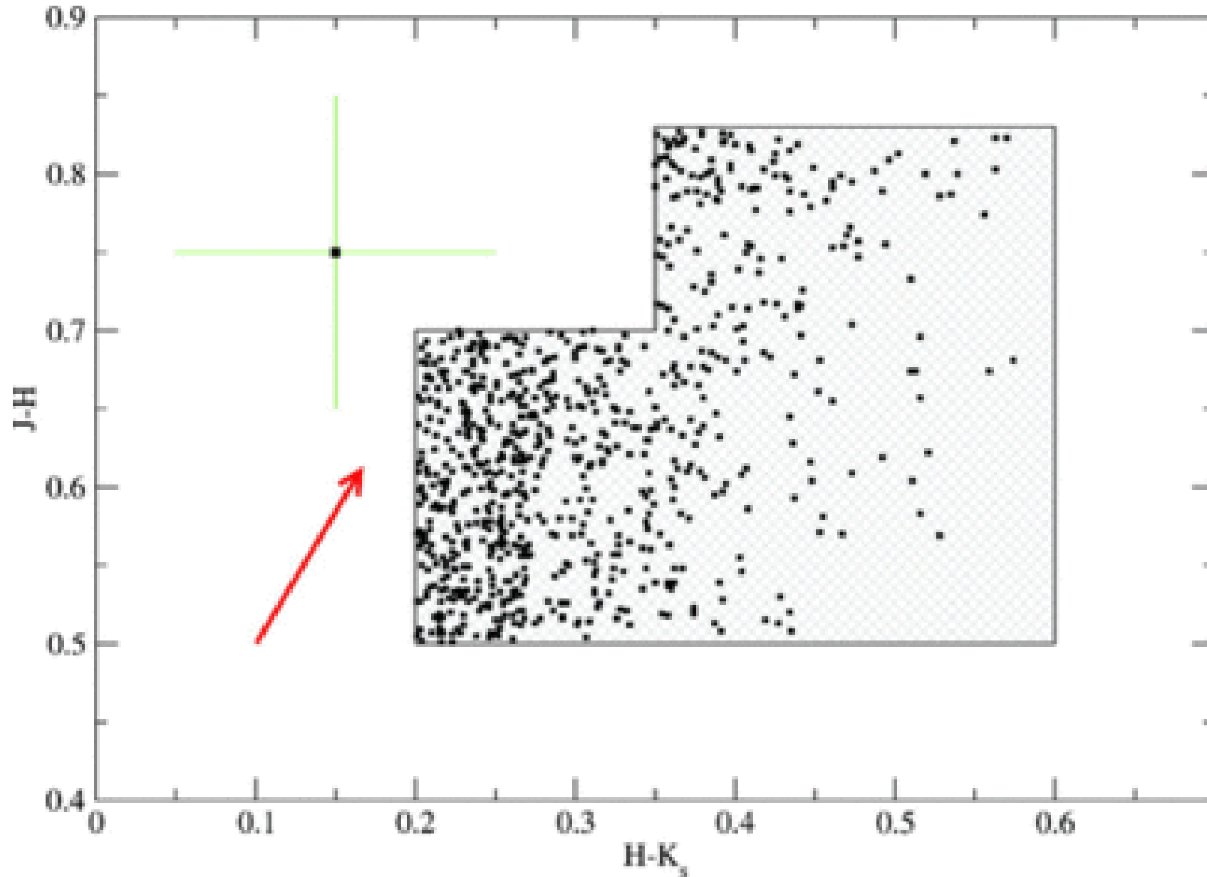
Fig. 2. from NearInfrared Variability in the 2MASS Calibration Fields: A Search for Planetary Transit Candidates Plavchan et al. 2008 ApJS 175 191 doi:10.1086/523644 https://dx.doi.org/10.1086/523644
