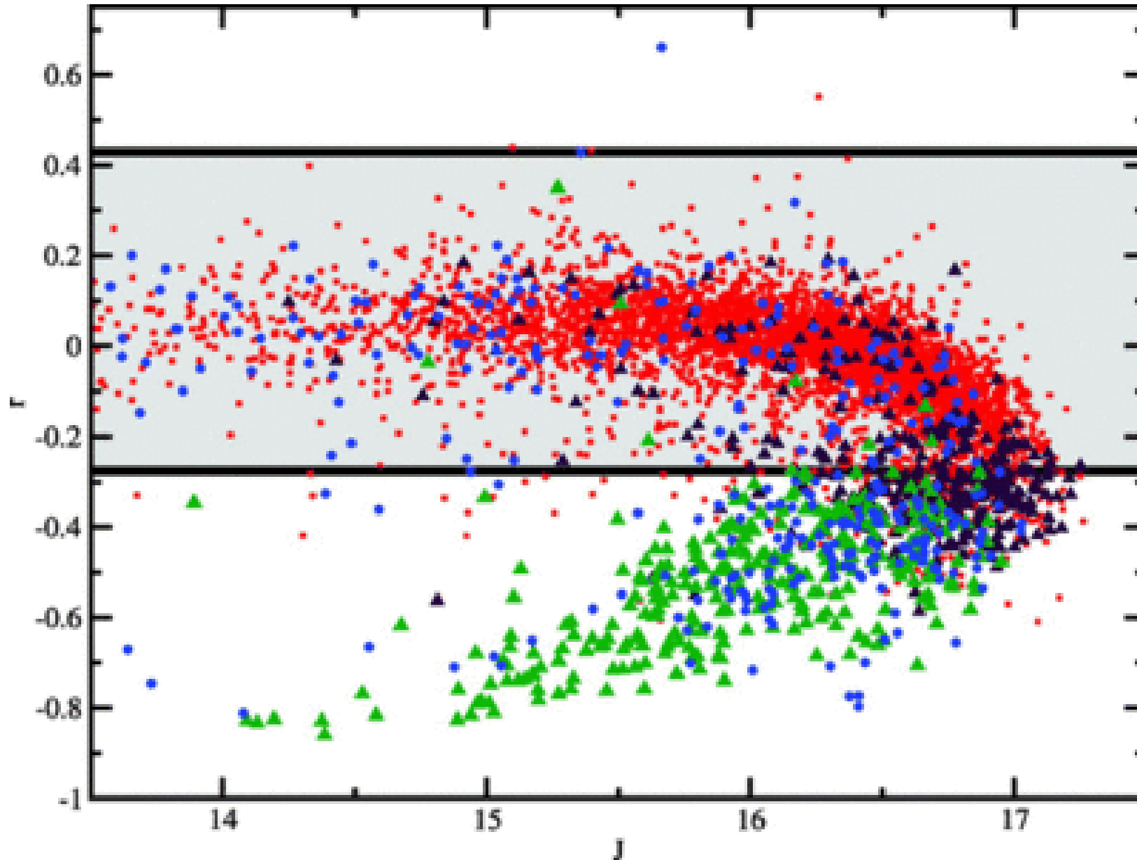
Fig. 15. from NearInfrared Variability in the 2MASS Calibration Fields: A Search for Planetary Transit Candidates Plavchan et al. 2008 ApJS 175 191 doi:10.1086/523644 https://dx.doi.org/10.1086/523644 © 2008. The American Astronomical Society. All rights reserved. Printed in U.S.A.
