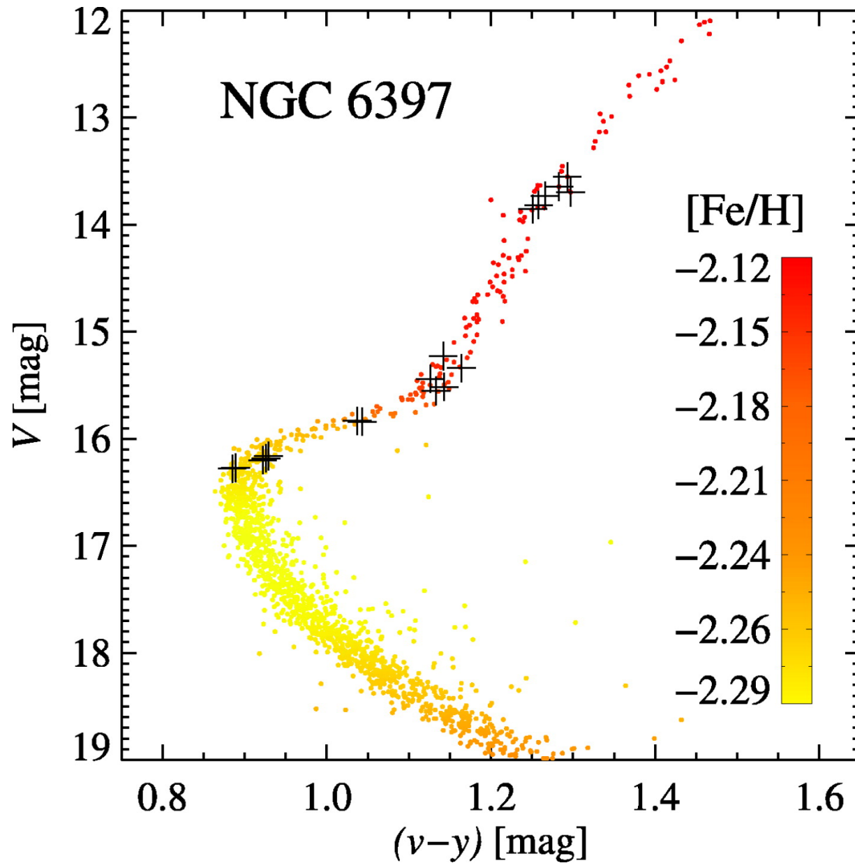
Fig. 9. from Atomic Diffusion and Mixing in Old Stars. I. Very Large Telescope FLAMESUUVES Observations of Stars in NGC 6397 Korn et al. 2007 ApJ 671 402 doi:10.1086/523098 https://dx.doi.org/10.1086/523098
