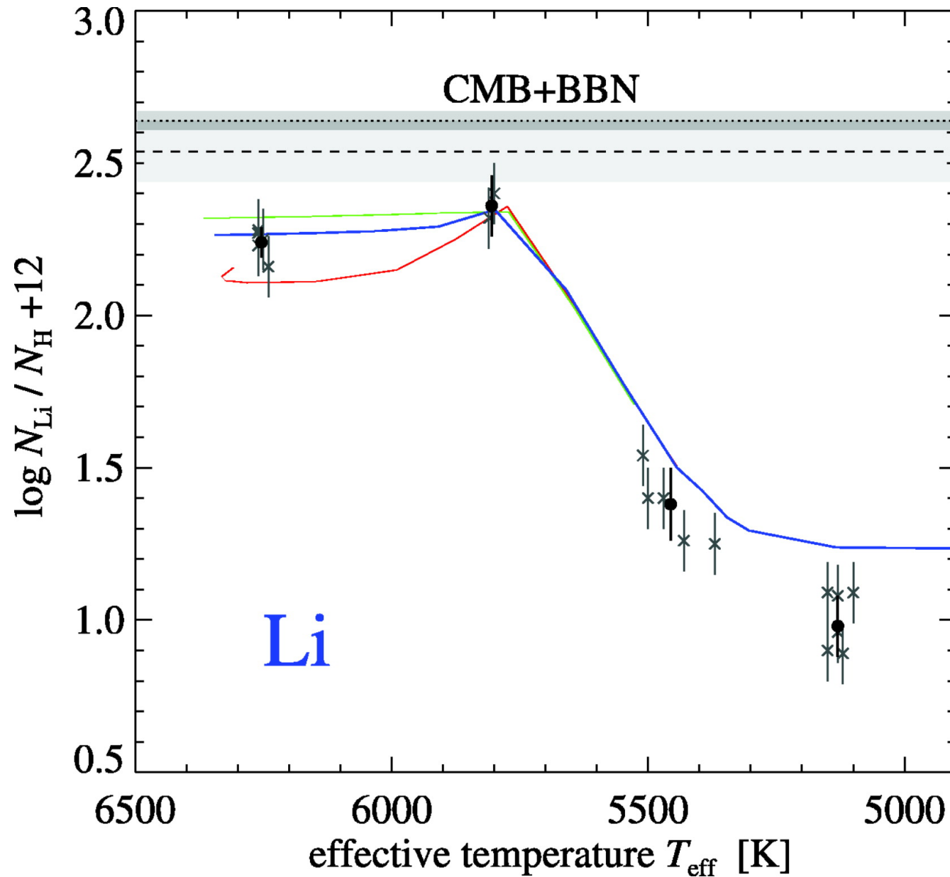
Fig. 8. from Atomic Diffusion and Mixing in Old Stars. I. Very Large Telescope FLAMESUVES Observations of Stars in NGC 6397 Korn et al. 2007 ApJ 671 402 doi:10.1086/523098 https://dx.doi.org/10.1086/523098
