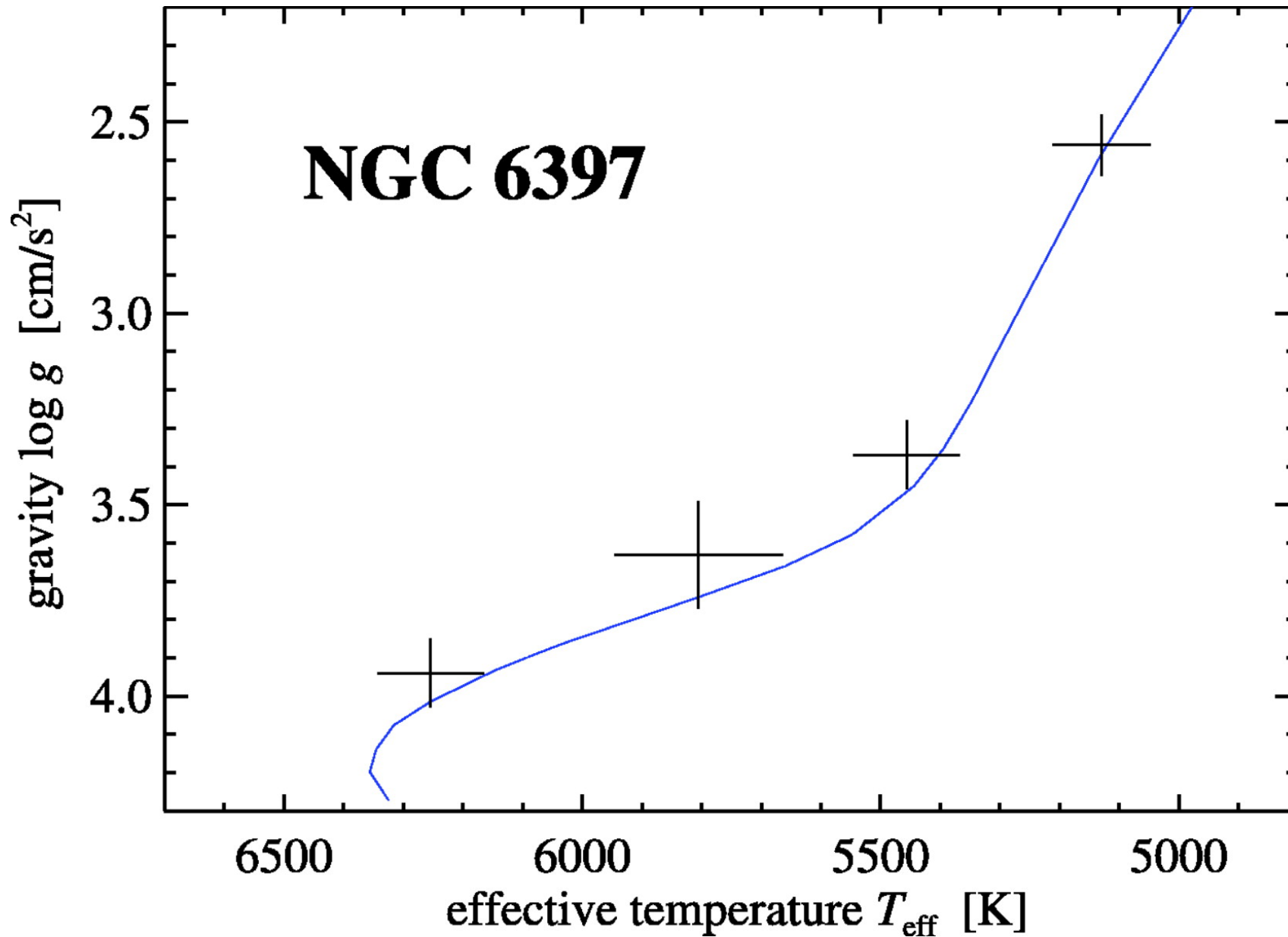
Fig. 7. from Atomic Diffusion and Mixing in Old Stars. I. Very Large Telescope FLAMESUVES Observations of Stars in NGC 6397 Korn et al. 2007 ApJ 671 402 doi:10.1086/523098 https://dx.doi.org/10.1086/523098 © 2007. The American Astronomical Society. All rights reserved. Printed in U.S.A.
