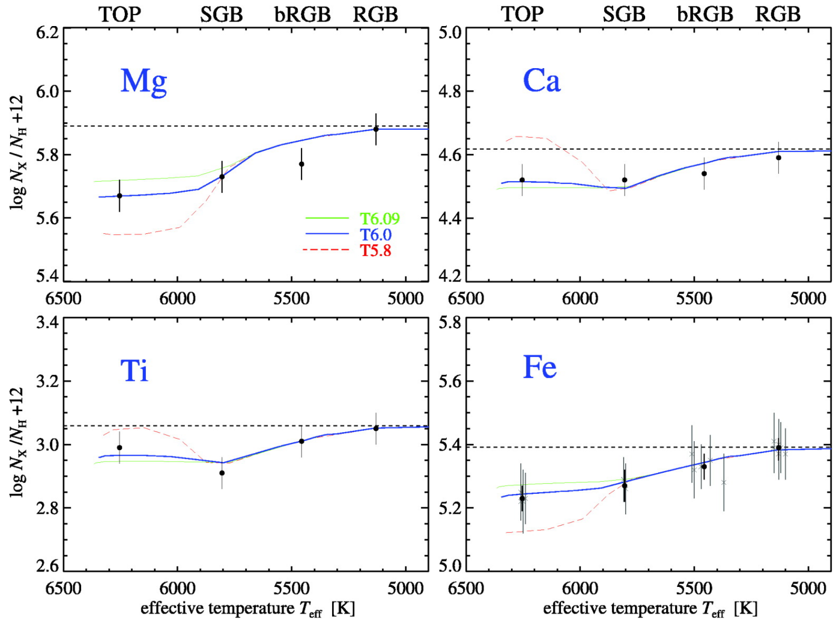
Fig. 6. from Atomic Diffusion and Mixing in Old Stars. I. Very Large Telescope FLAMES/UVES Observations of Stars in NGC 6397 Korn et al. 2007 ApJ 671 402 doi:10.1086/523098 https://dx.doi.org/10.1086/523098
