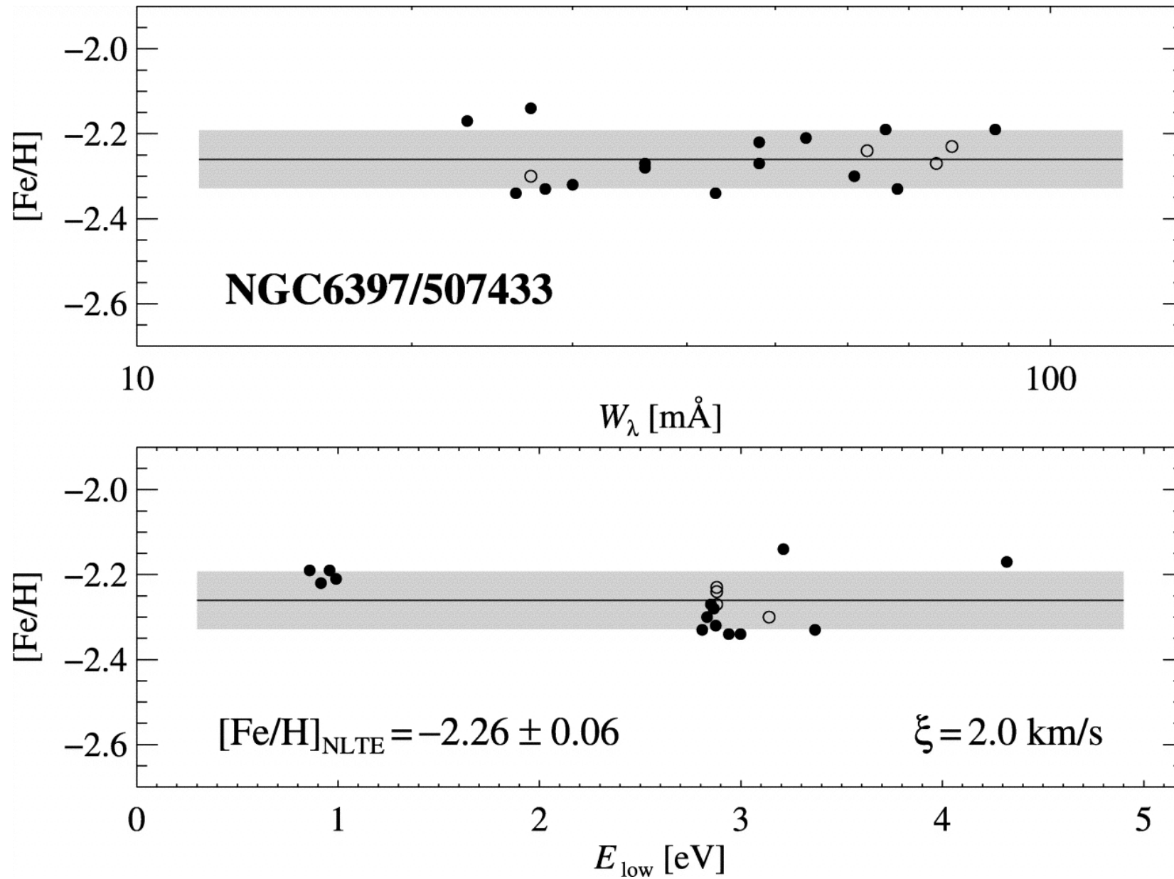
Fig. 5. from Atomic Diffusion and Mixing in Old Stars. I. Very Large Telescope FLAMESUVES Observations of Stars in NGC 6397 Korn et al. 2007 ApJ 671 402 doi:10.1086/523098 https://dx.doi.org/10.1086/523098 © 2007. The American Astronomical Society. All rights reserved. Printed in U.S.A.
