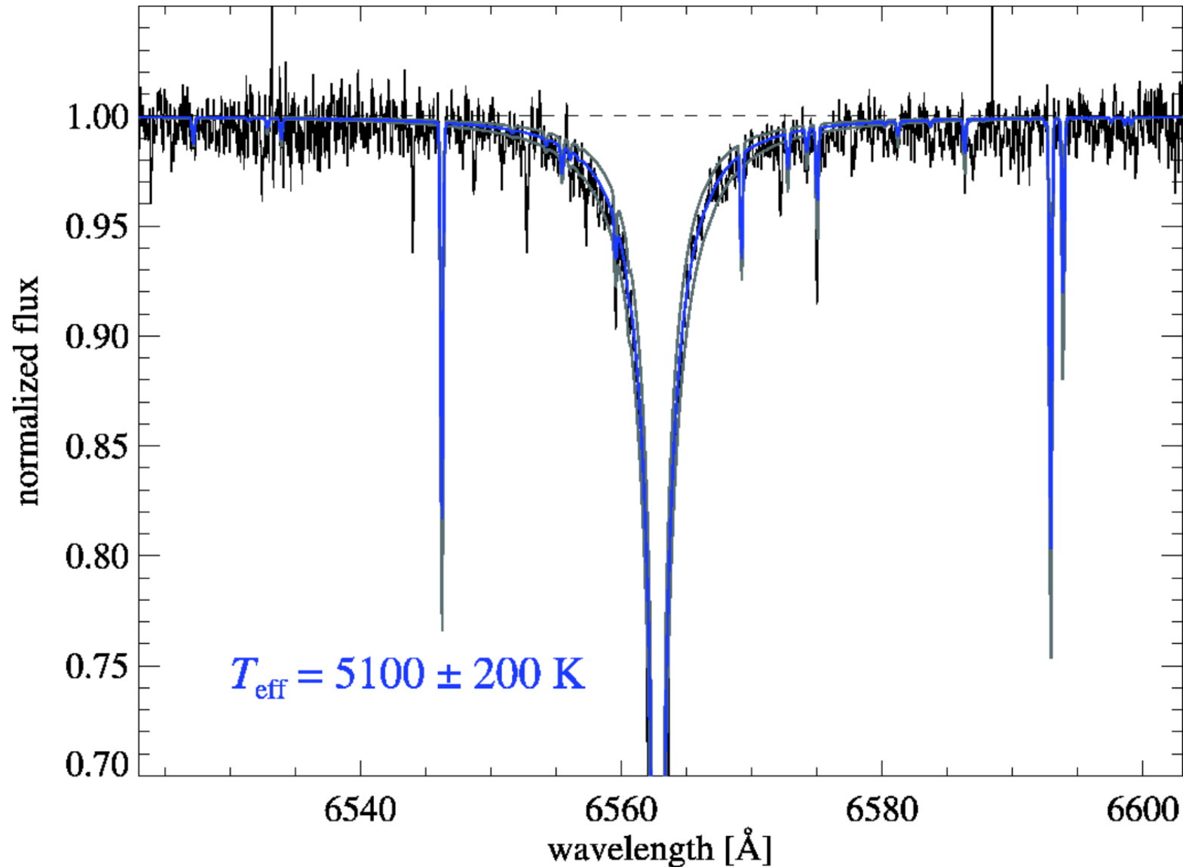
Fig. 4. from Atomic Diffusion and Mixing in Old Stars. I. Very Large Telescope FLAMESUVES Observations of Stars in NGC 6397 Korn et al. 2007 ApJ 671 402 doi:10.1086/523098 https://dx.doi.org/10.1086/523098 © 2007. The American Astronomical Society. All rights reserved. Printed in U.S.A.
