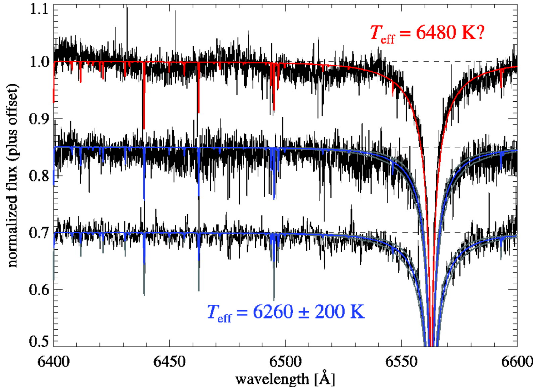
Fig. 3. from Atomic Diffusion and Mixing in Old Stars. I. Very Large Telescope FLAMES/UVES Observations of Stars in NGC 6397 Korn et al. 2007 ApJ 671 402 doi:10.1086/523098 https://dx.doi.org/10.1086/523098 © 2007. The American Astronomical Society. All rights reserved. Printed in U.S.A.
