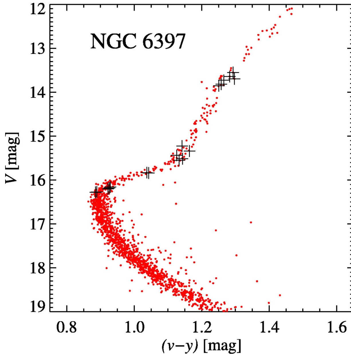
Fig. 2. from Atomic Diffusion and Mixing in Old Stars. I. Very Large Telescope FLAMESUVES Observations of Stars in NGC 6397 Korn et al. 2007 ApJ 671 402 doi:10.1086/523098 https://dx.doi.org/10.1086/523098
