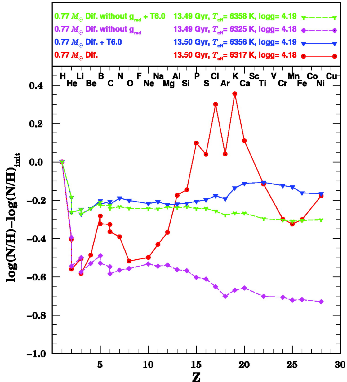
Fig. 1. from Atomic Diffusion and Mixing in Old Stars. I. Very Large Telescope FLAMESUVES Observations of Stars in NGC 6397 Korn et al. 2007 ApJ 671 402 doi:10.1086/523098 https://dx.doi.org/10.1086/523098 © 2007. The American Astronomical Society. All rights reserved. Printed in U.S.A.
