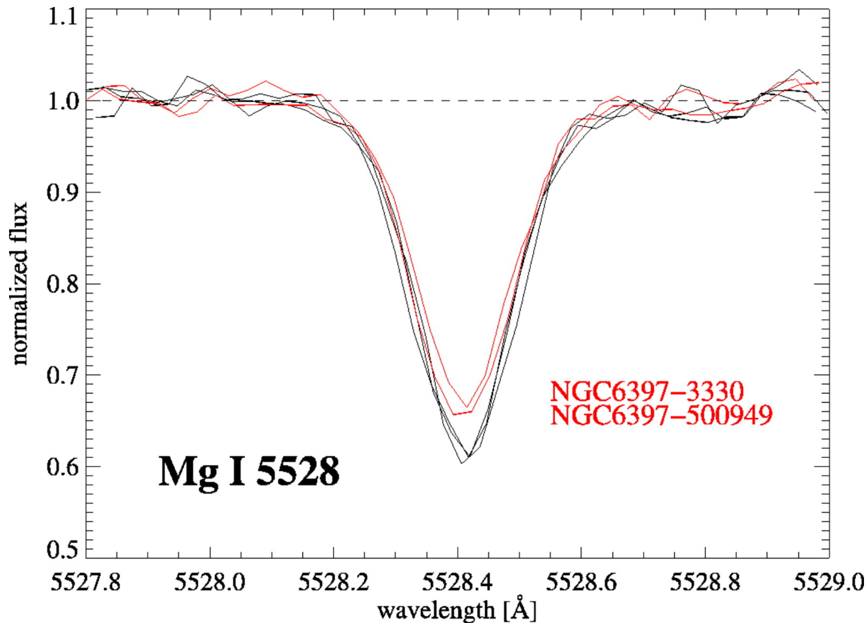
Fig. 11. from Atomic Diffusion and Mixing in Old Stars. I. Very Large Telescope FLAMESUVES Observations of Stars in NGC 6397 Korn et al. 2007 ApJ 671 402 doi:10.1086/523098 https://dx.doi.org/10.1086/523098
