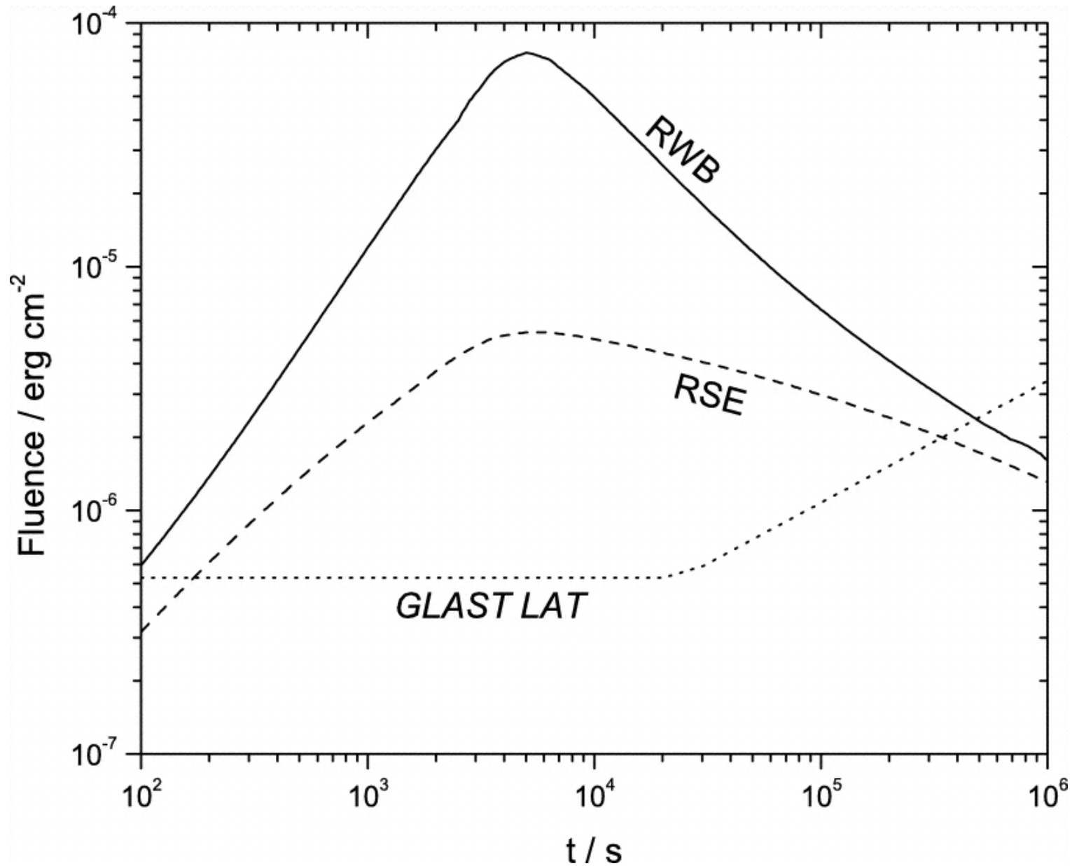
Fig. 7. from Observational Signatures of HighEnergy Emission during the Shallow Decay Phase of GammaRay Burst XRay Afterglows Yu, Liu, & Dai 2007 ApJ 671 637 doi:10.1086/522829 https://dx.doi.org/10.1086/522829
