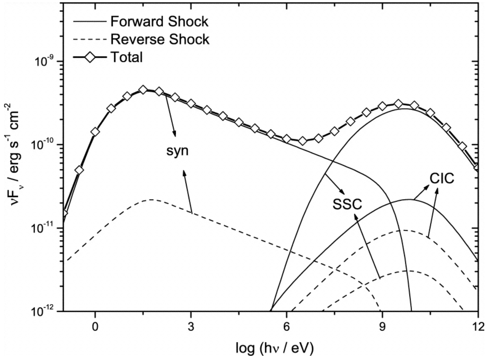
Fig. 6. from Observational Signatures of HighEnergy Emission during the Shallow Decay Phase of GammaRay Burst XRay Afterglows Yu, Liu, & Dai 2007 ApJ 671 637 doi:10.1086/522829 https://dx.doi.org/10.1086/522829 © 2007. The American Astronomical Society. All rights reserved. Printed in U.S.A.
