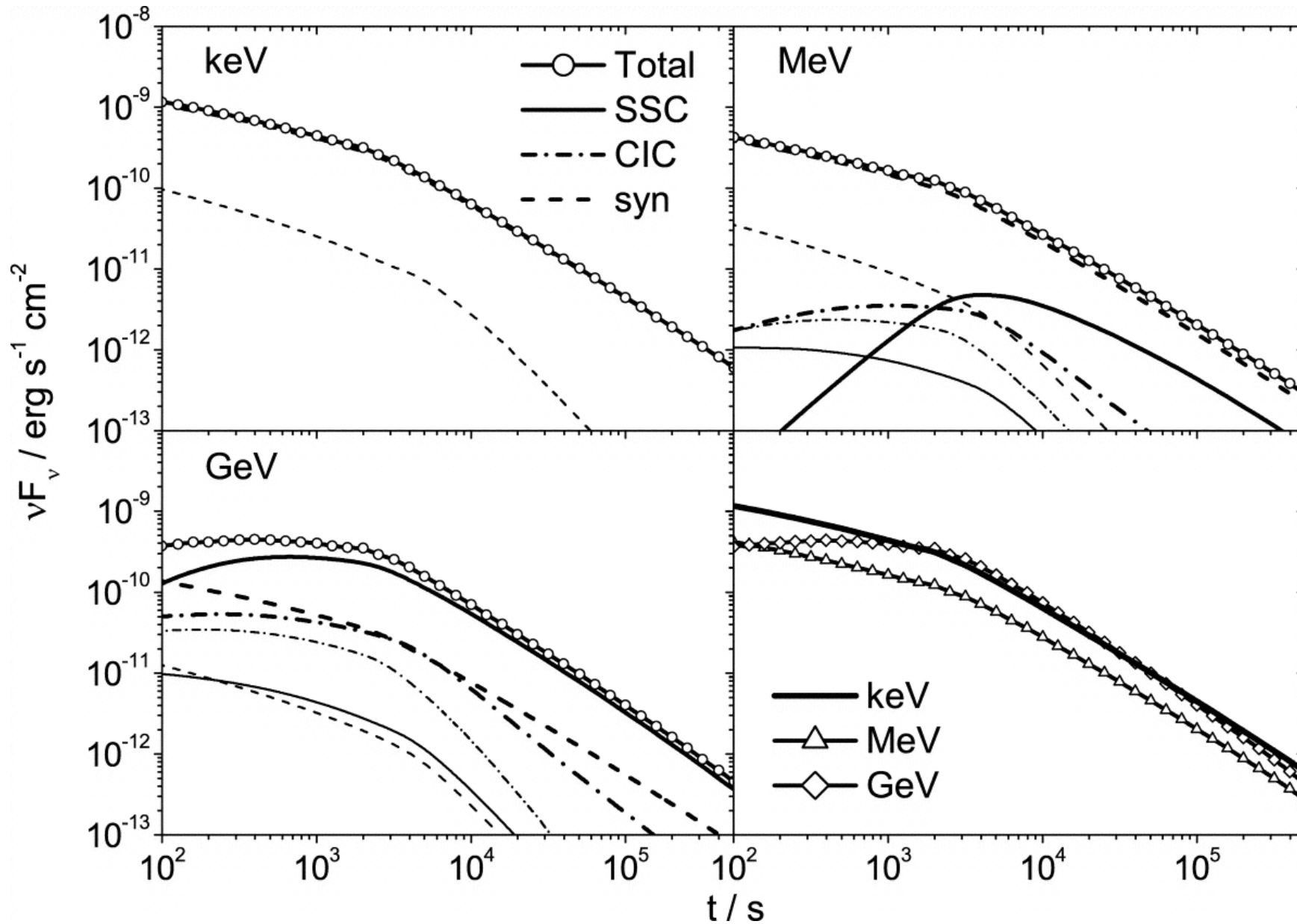
Fig. 5. from Observational Signatures of HighEnergy Emission during the Shallow Decay Phase of GammaRay Burst XRay Afterglows Yu, Liu, & Dai 2007 ApJ 671 637 doi:10.1086/522829 https://dx.doi.org/10.1086/522829
