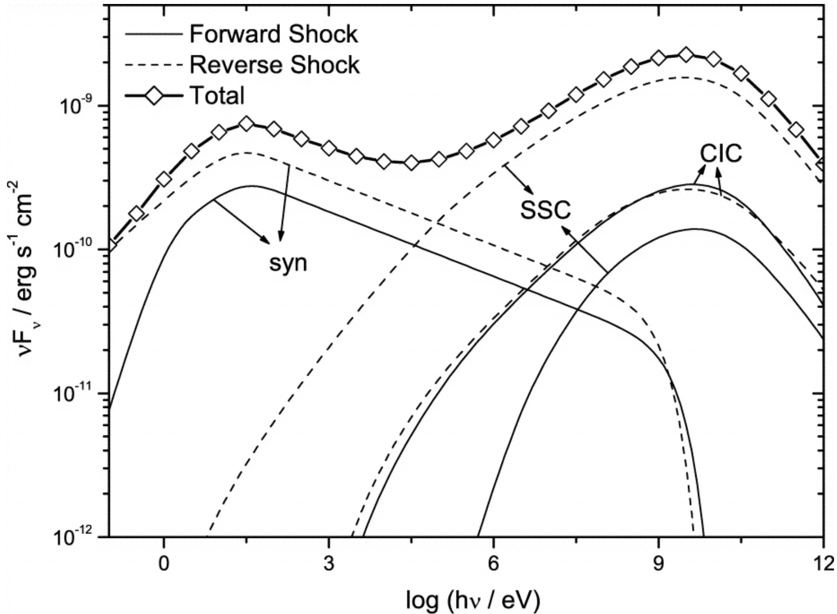
Fig. 4. from Observational Signatures of HighEnergy Emission during the Shallow Decay Phase of GammaRay Burst XRay Afterglows Yu, Liu, & Dai 2007 ApJ 671 637 doi:10.1086/522829 https://dx.doi.org/10.1086/522829 © 2007. The American Astronomical Society. All rights reserved. Printed in U.S.A.
