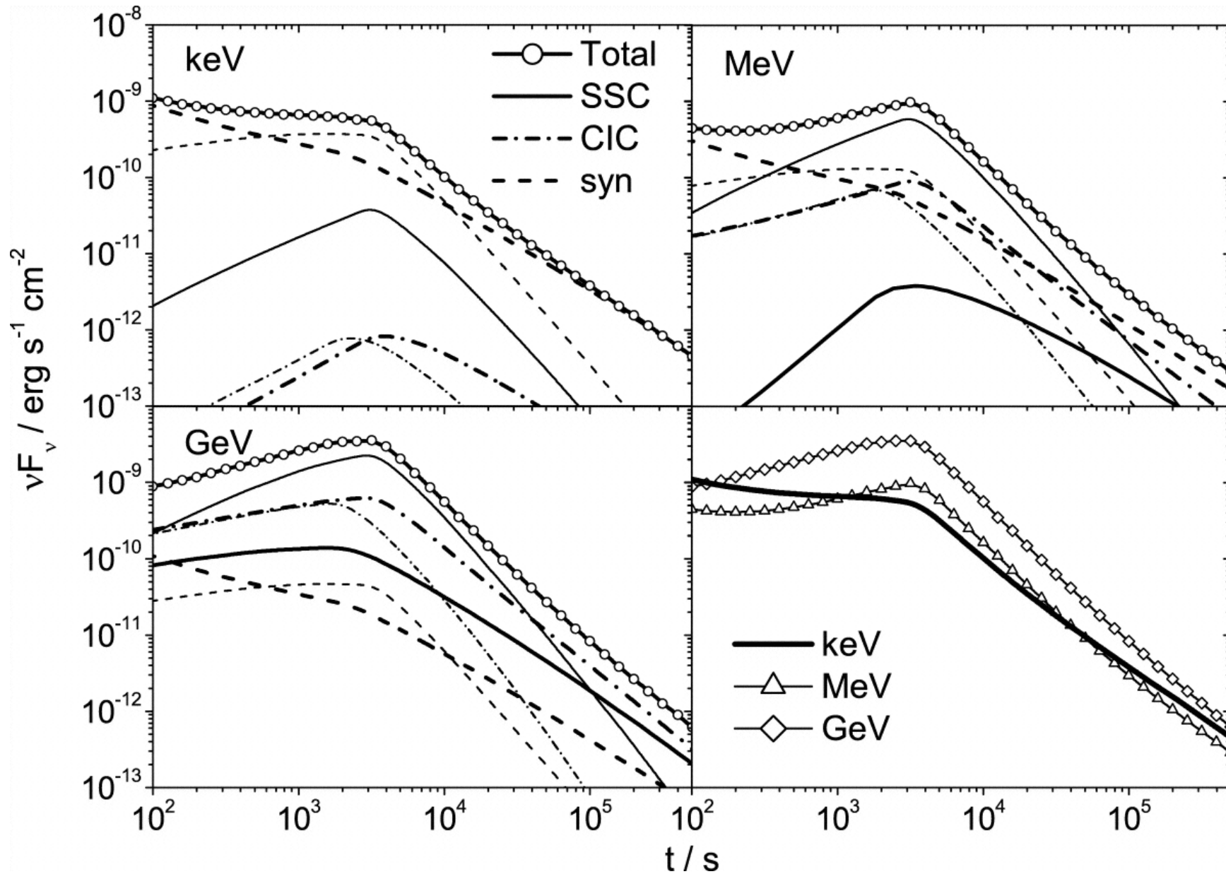
Fig. 3. from Observational Signatures of HighEnergy Emission during the Shallow Decay Phase of GammaRay Burst XRay Afterglows Yu, Liu, & Dai 2007 ApJ 671 637 doi:10.1086/522829 https://dx.doi.org/10.1086/522829
