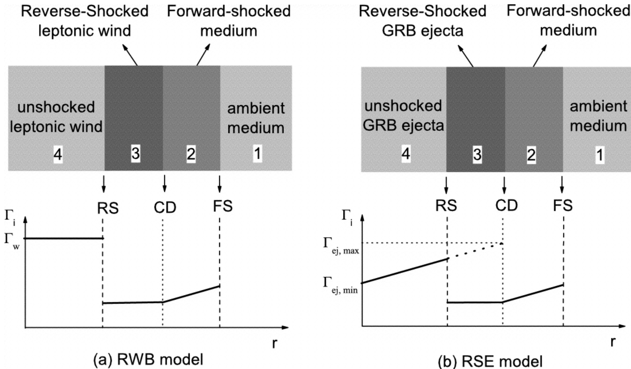
Fig. 1. from Observational Signatures of HighEnergy Emission during the Shallow Decay Phase of GammaRay Burst XRay Afterglows Yu, Liu, & Dai 2007 ApJ 671 637 doi:10.1086/522829 https://dx.doi.org/10.1086/522829
