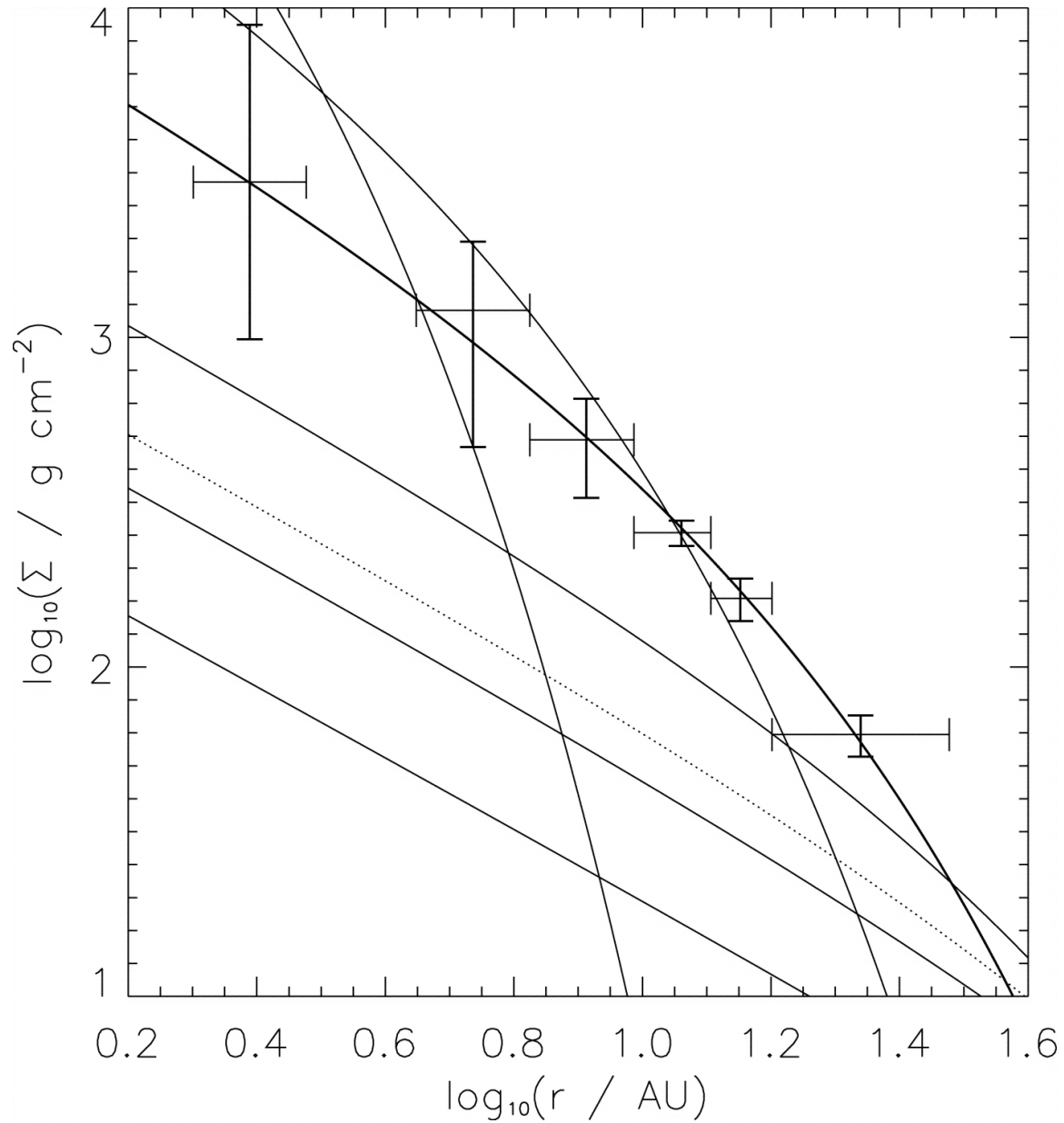
Fig. 2. from Mass Distribution and Planet Formation in the Solar Nebula Desch 2007 ApJ 671 878 doi:10.1086/522825 https://dx.doi.org/10.1086/522825 © 2007. The American Astronomical Society. All rights reserved. Printed in U.S.A.
