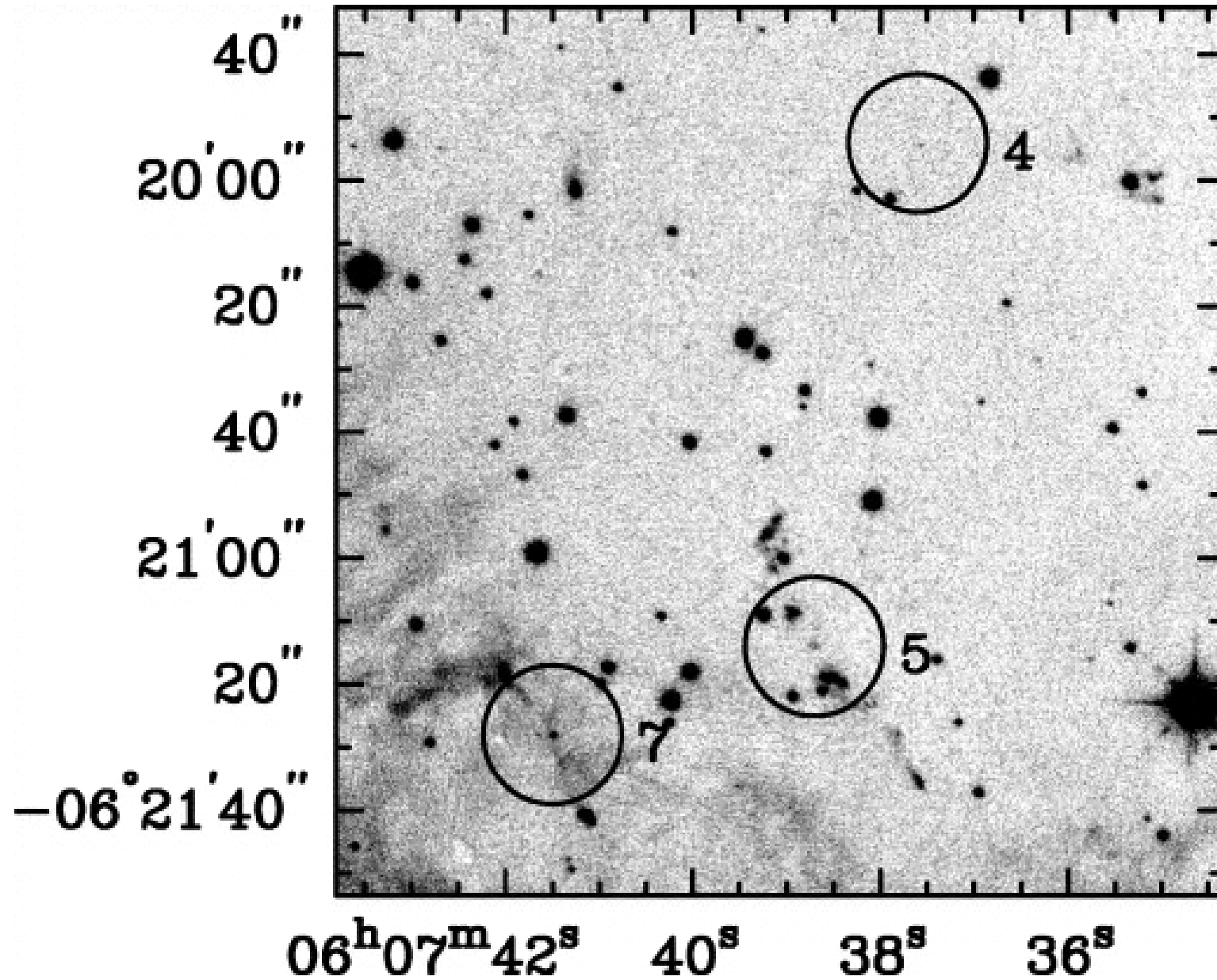
Fig. 7. from New H 2 Jets in Monoceros R2 Hodapp 2007 AJ 134 2020 doi:10.1086/522784 https://dx.doi.org/10.1086/522784
