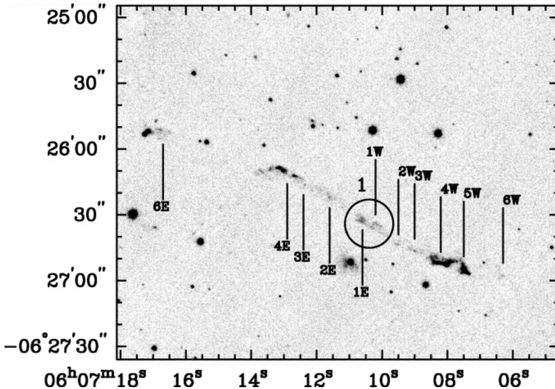
Fig. 4. from New H 2 Jets in Monoceros R2 Hodapp 2007 AJ 134 2020 doi:10.1086/522784 https://dx.doi.org/10.1086/522784
