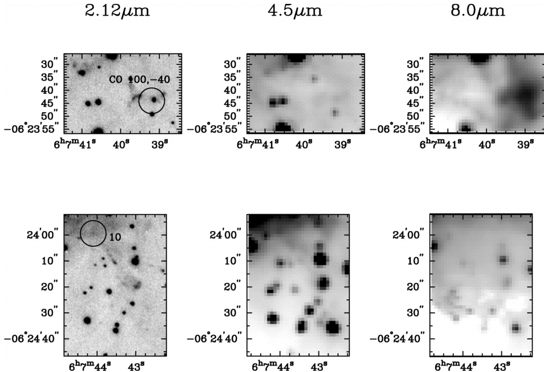
Fig. 3. from New H 2 Jets in Monoceros R2 Hodapp 2007 AJ 134 2020 doi:10.1086/522784 https://dx.doi.org/10.1086/522784
