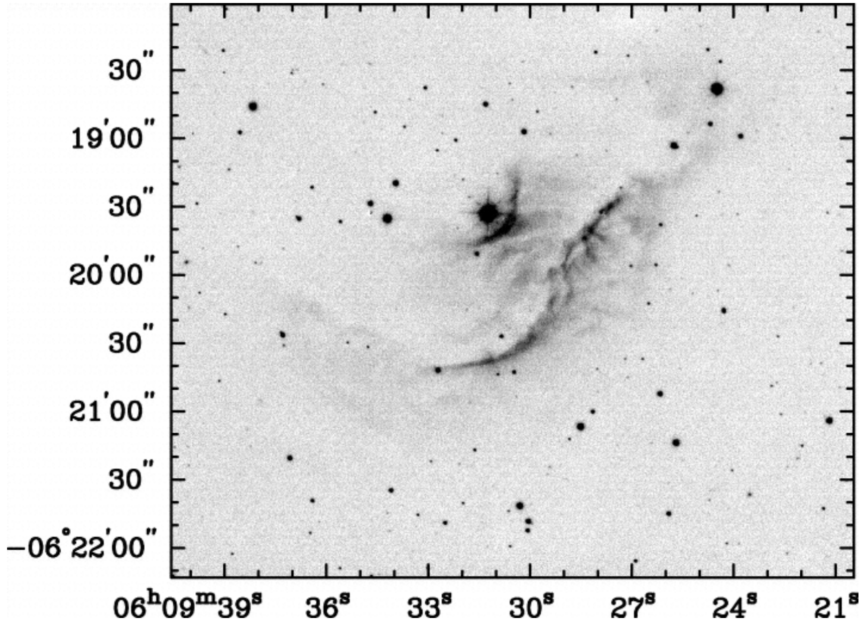
Fig. 19. from New H 2 Jets in Monoceros R2 Hodapp 2007 AJ 134 2020 doi:10.1086/522784 https://dx.doi.org/10.1086/522784
