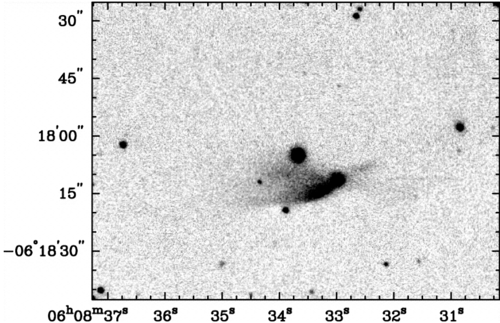
Fig. 18. from New H 2 Jets in Monoceros R2 Hodapp 2007 AJ 134 2020 doi:10.1086/522784 https://dx.doi.org/10.1086/522784
