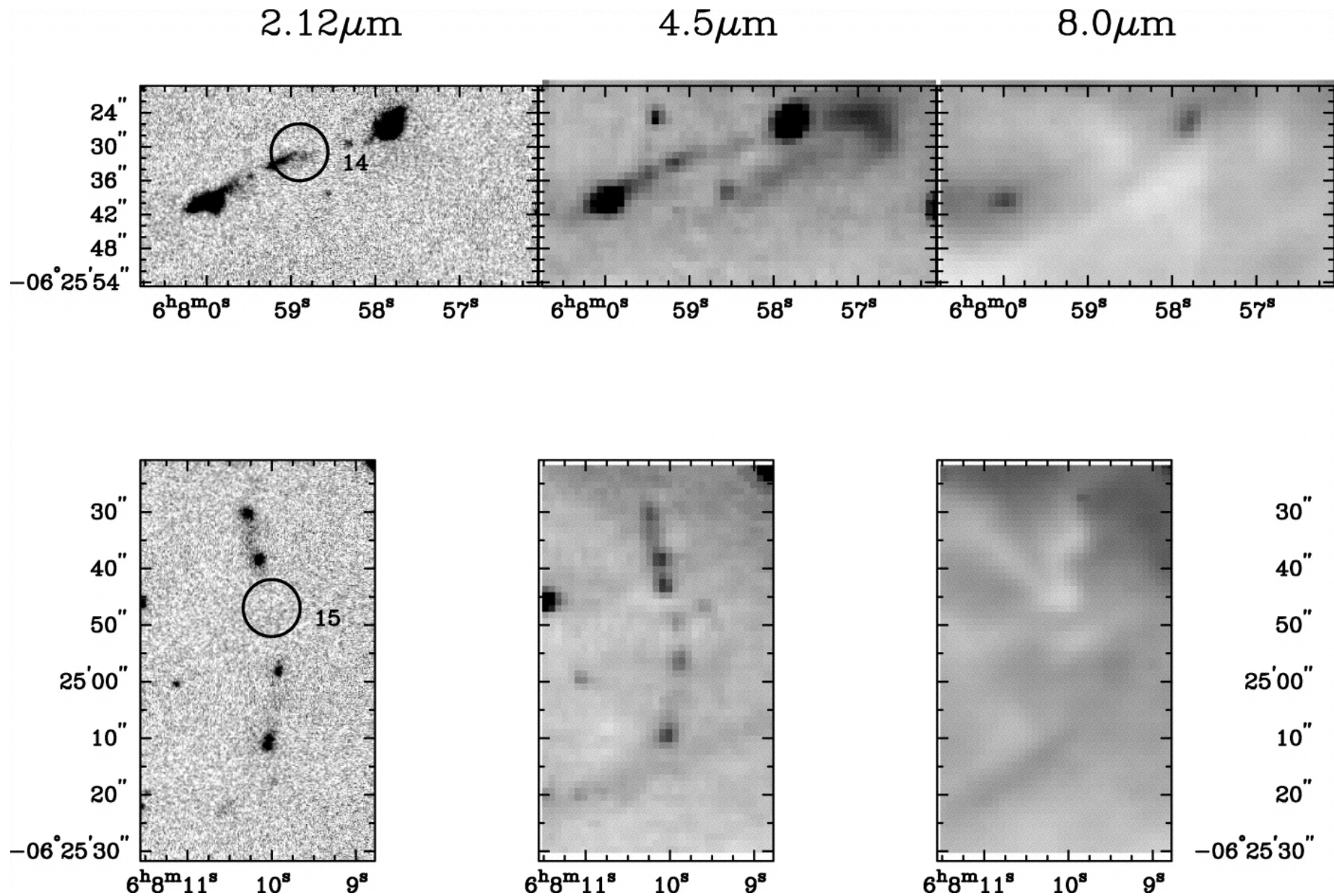
Fig. 16. from New H 2 Jets in Monoceros R2 Hodapp 2007 AJ 134 2020 doi:10.1086/522784 https://dx.doi.org/10.1086/522784
