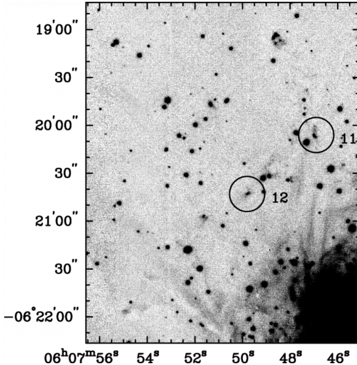
Fig. 11. from New H 2 Jets in Monoceros R2 Hodapp 2007 AJ 134 2020 doi:10.1086/522784 https://dx.doi.org/10.1086/522784
