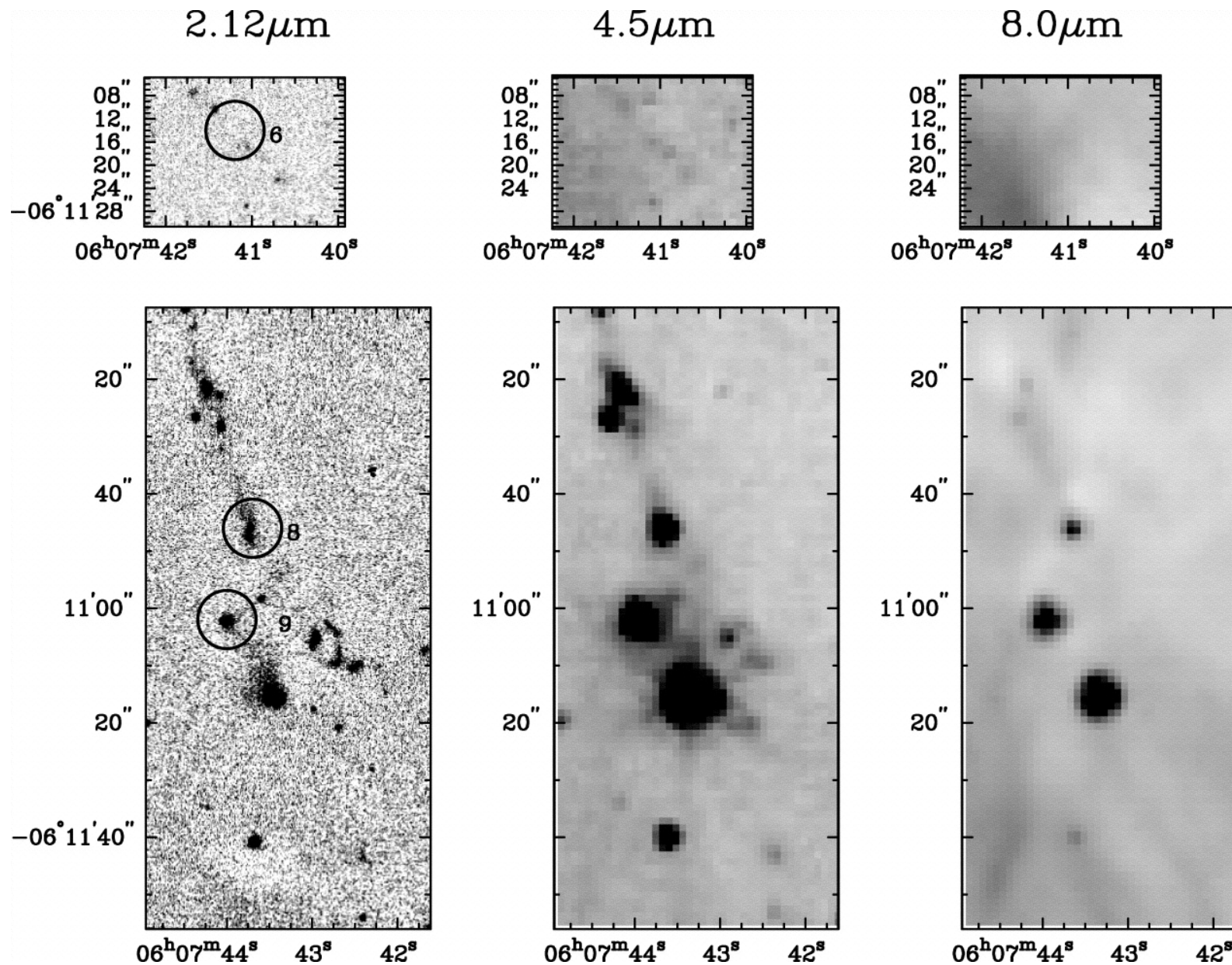
Fig. 10. from New H2 Jets in Monoceros R2 Hodapp 2007 AJ 134 2020 doi:10.1086/522784 https://dx.doi.org/10.1086/522784
