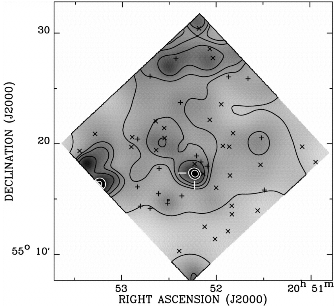
Fig. 3. from The Chandra View of DA 530: A Subenergetic Supernova Remnant with a Pulsar Wind Nebula? Jiang, Chen, & Wang 2007 ApJ 670 1142 doi:10.1086/522299 https://dx.doi.org/10.1086/522299 © 2007. The American Astronomical Society. All rights reserved. Printed in U.S.A.
