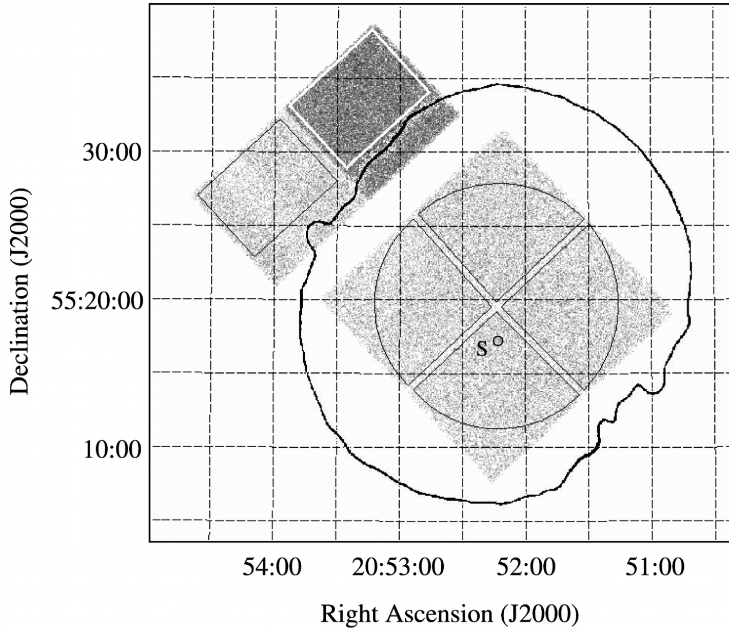
Fig. 1. from The Chandra View of DA 530: A Subenergetic Supernova Remnant with a Pulsar Wind Nebula? Jiang, Chen, & Wang 2007 ApJ 670 1142 doi:10.1086/522299 https://dx.doi.org/10.1086/522299 © 2007. The American Astronomical Society. All rights reserved. Printed in U.S.A.
