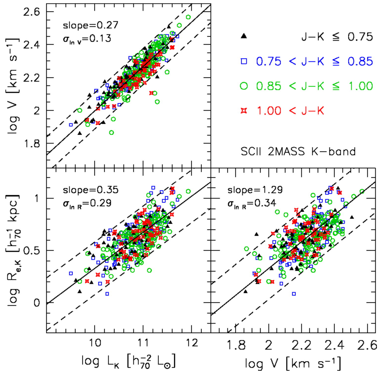
Fig. 9. from Scaling Relations of Spiral Galaxies Courteau et al. 2007 ApJ 671 203 doi:10.1086/522193 https://dx.doi.org/10.1086/522193
