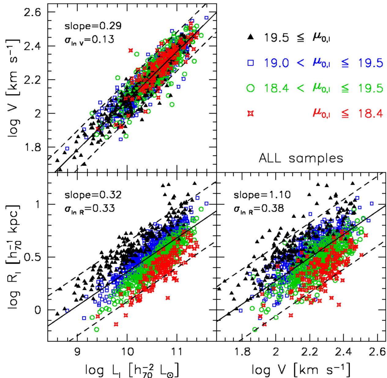
Fig. 6. from Scaling Relations of Spiral Galaxies Courteau et al. 2007 ApJ 671 203 doi:10.1086/522193 https://dx.doi.org/10.1086/522193
